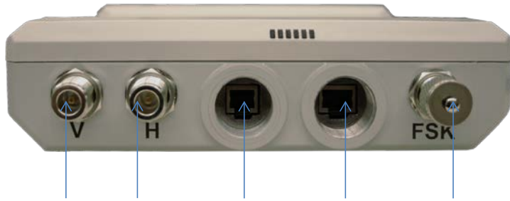
Figure 5 AP interfaces - 5 GHz original layout
