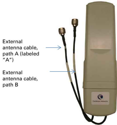
Figure 11 Connectorized SM
