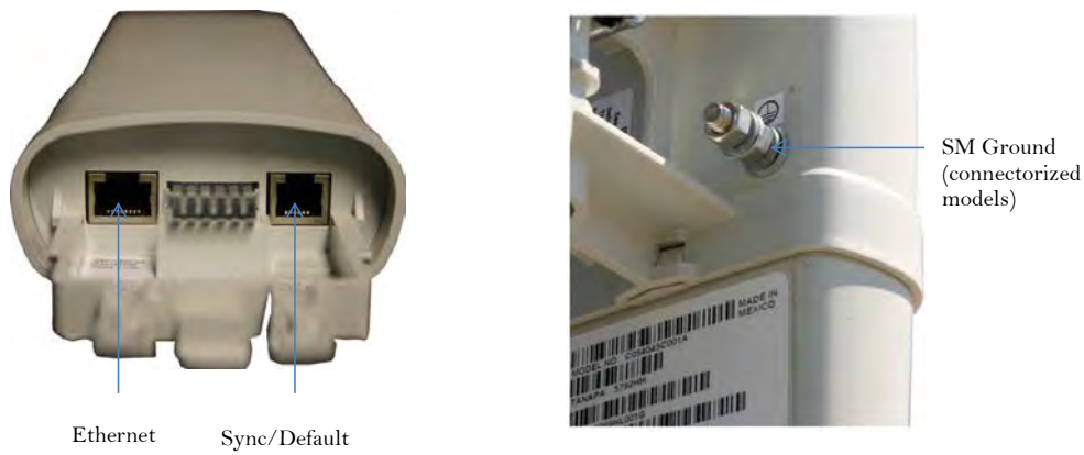
Figure 10 SM interfaces
