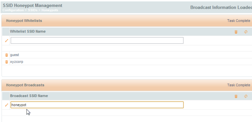
Figure 152. Honeypot Whitelist
