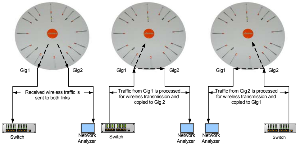
Figure 91. Port Modes (e-f)
