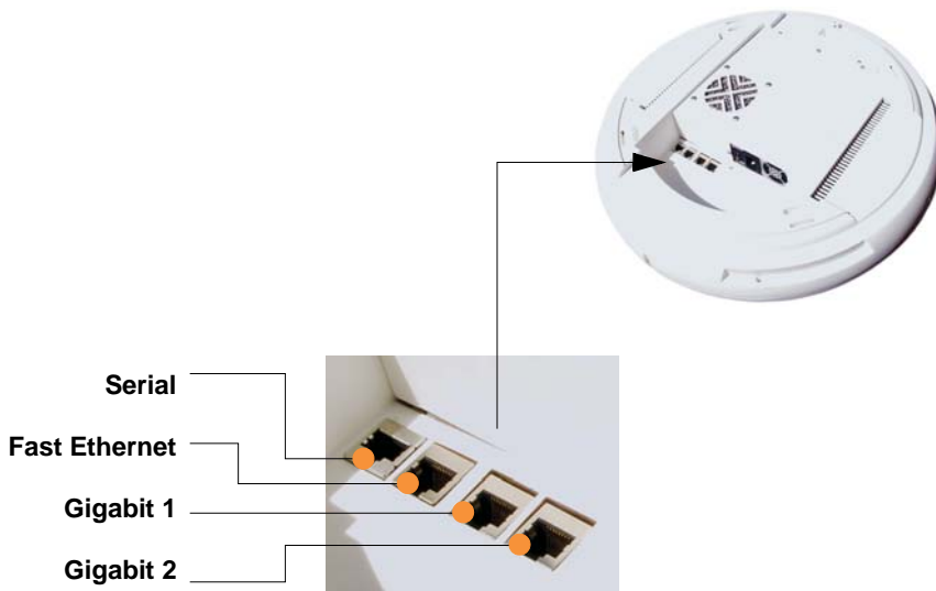
Figure 88. Network Interface Ports
