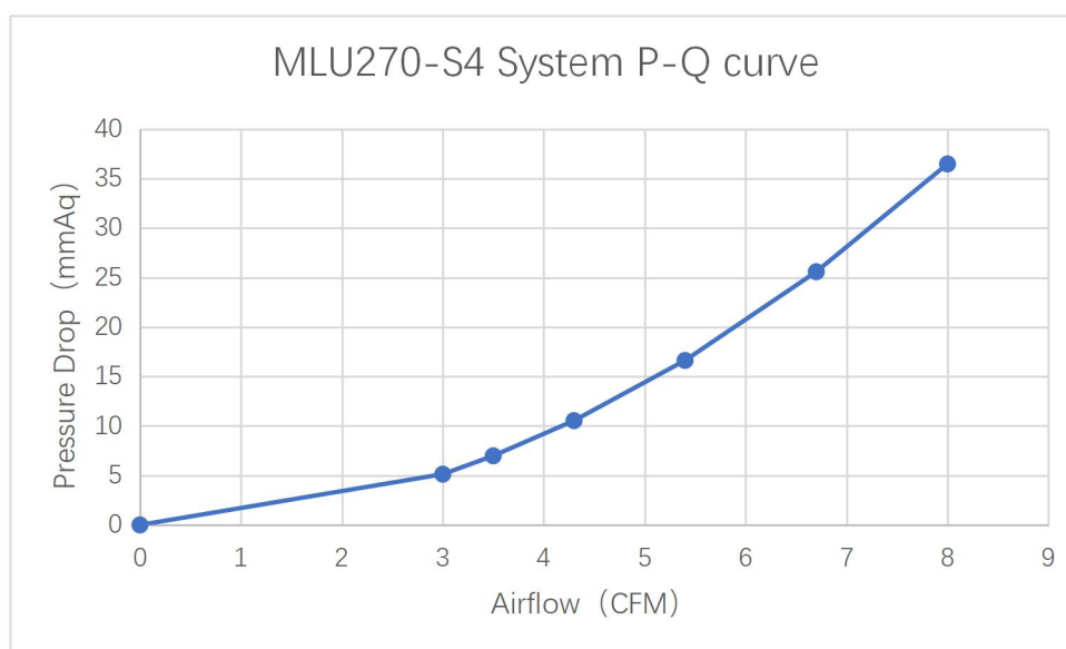
Figure.4 MLU270-S System Pressure Drop
