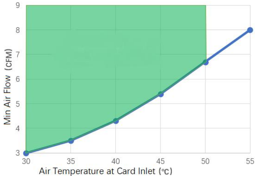
Figure.6 Air Inlet Temperature vs Min Airflow Requirement
