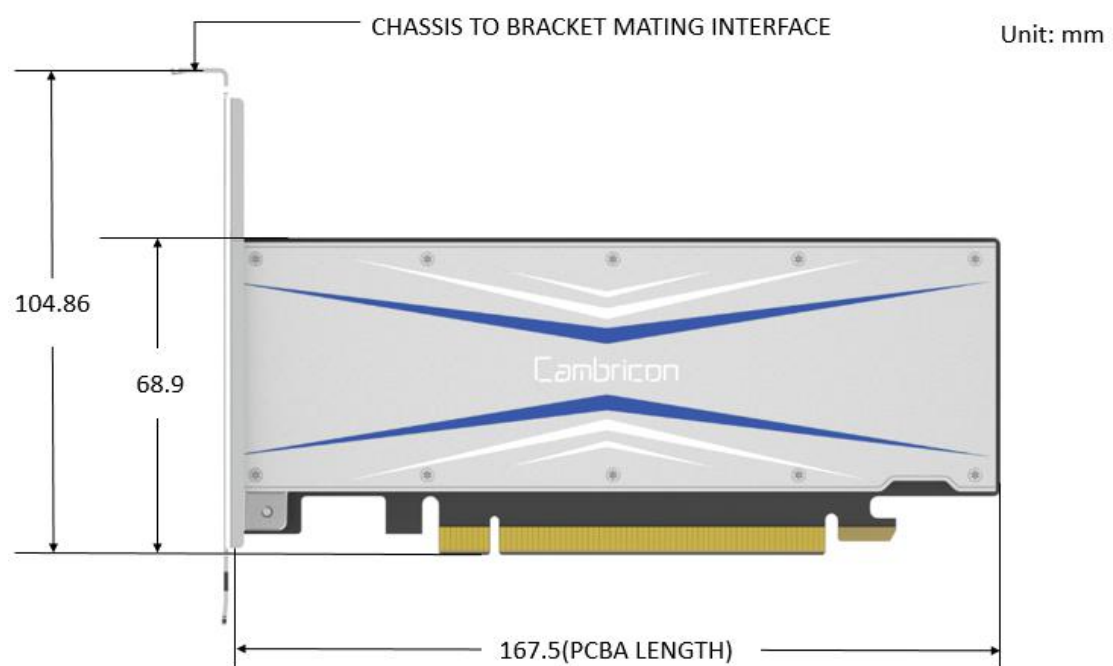
Figure. 2 MLU270-S Series Intelligent Processing Card Dimensions (High bracket)
