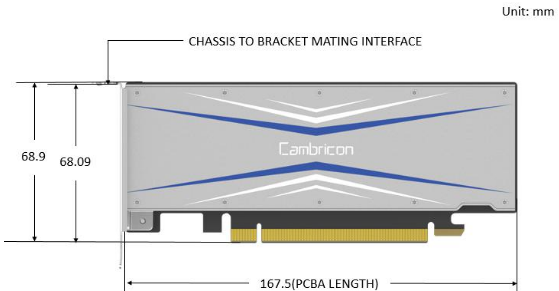
Figure. 2 MLU270-S Series Intelligent Processing Card Dimensions (High bracket)
