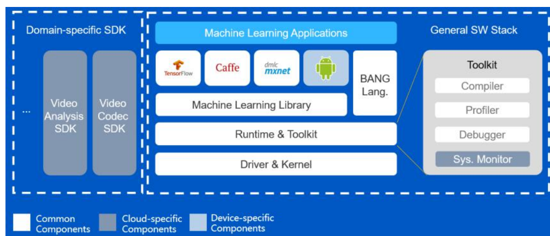
Figure.7 Cambricon NeuWare
