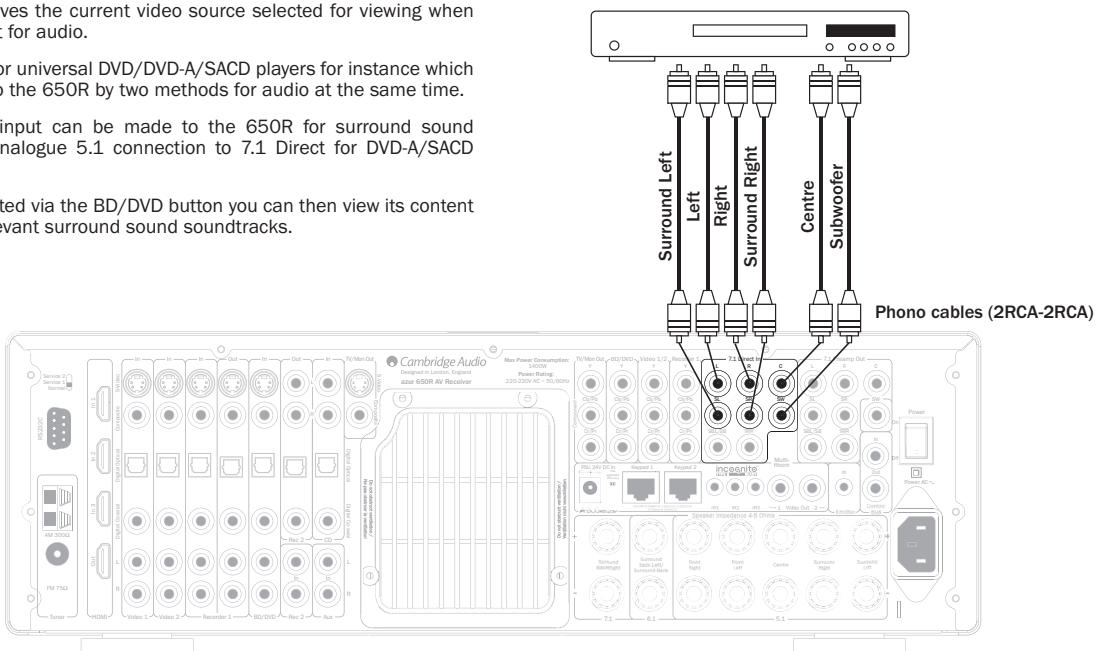
DVD-A player or SACD multi-channel player 5.1 connections
