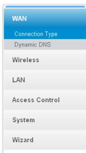
Figure 11. Configuration Menu
