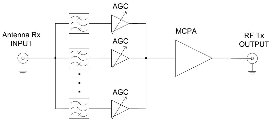
Figure 1 – UHF Narrowband Signal Booster Basic Block Diagram
