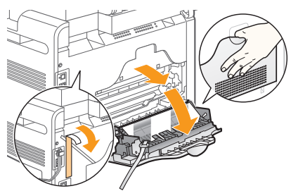
2 Remove the tape. 3 Open the rear cover.
