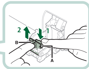
Saddle Stitcher Unit of the Booklet Finisher-G1 (p. 142)
