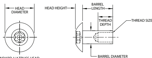
STANDARD 1/4 TRUSS HEAD TAMPER RESISTANT 6-LOBE T27 DRIVE GO GAGE PENETRATION: .070 MIN.
