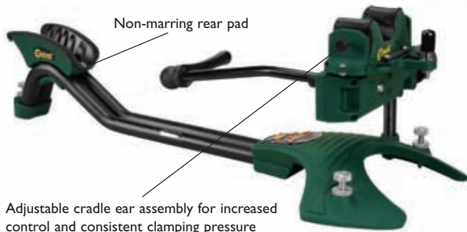
Fire Control Full Length Rest package: 24.8" wide x 12.6" high x 9.3" deep
