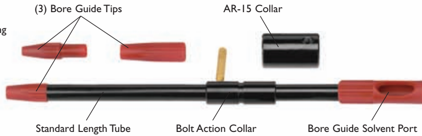
Universal Bore Guide Kit package: 4.75" wide x 16.5" high x 1.5" deep
