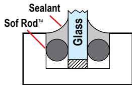
Sof Rod™ for Glazing
