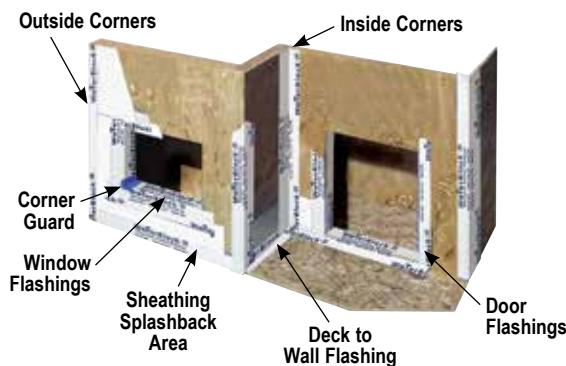
Typical Corner Guard Installation
