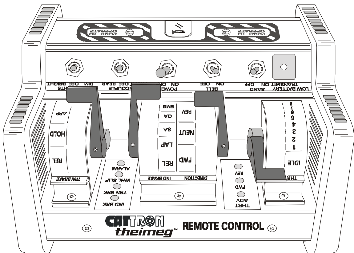
Figure 3-6. Locomotive Paddle Controller - Typical Configuration
