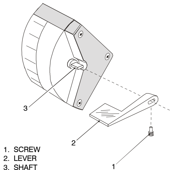
Figure 4-4. Lever Replacement.
