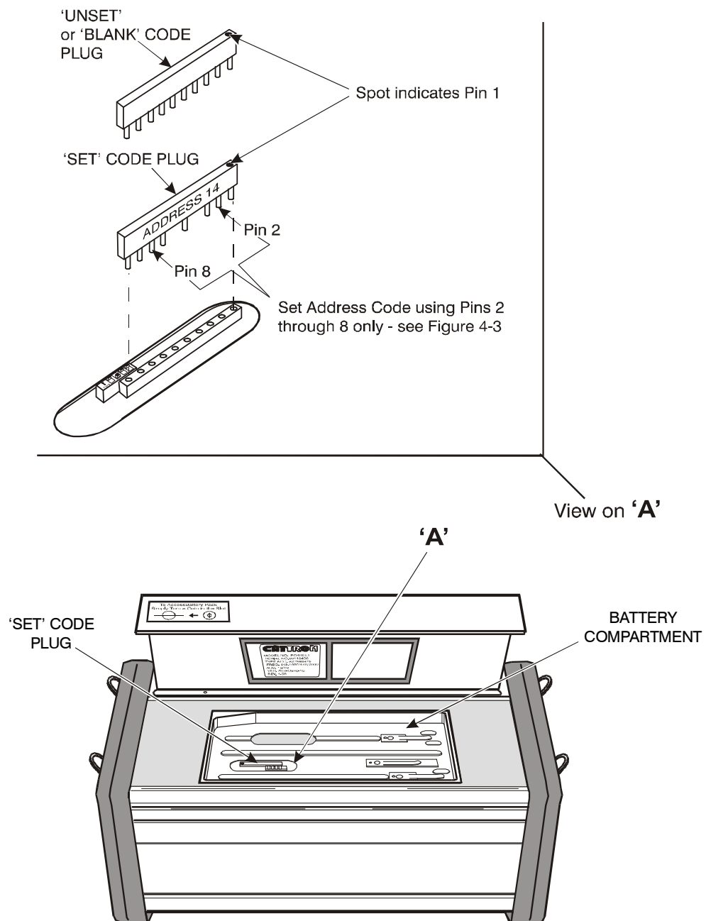
Figure 4-2. Code Plug Location.
