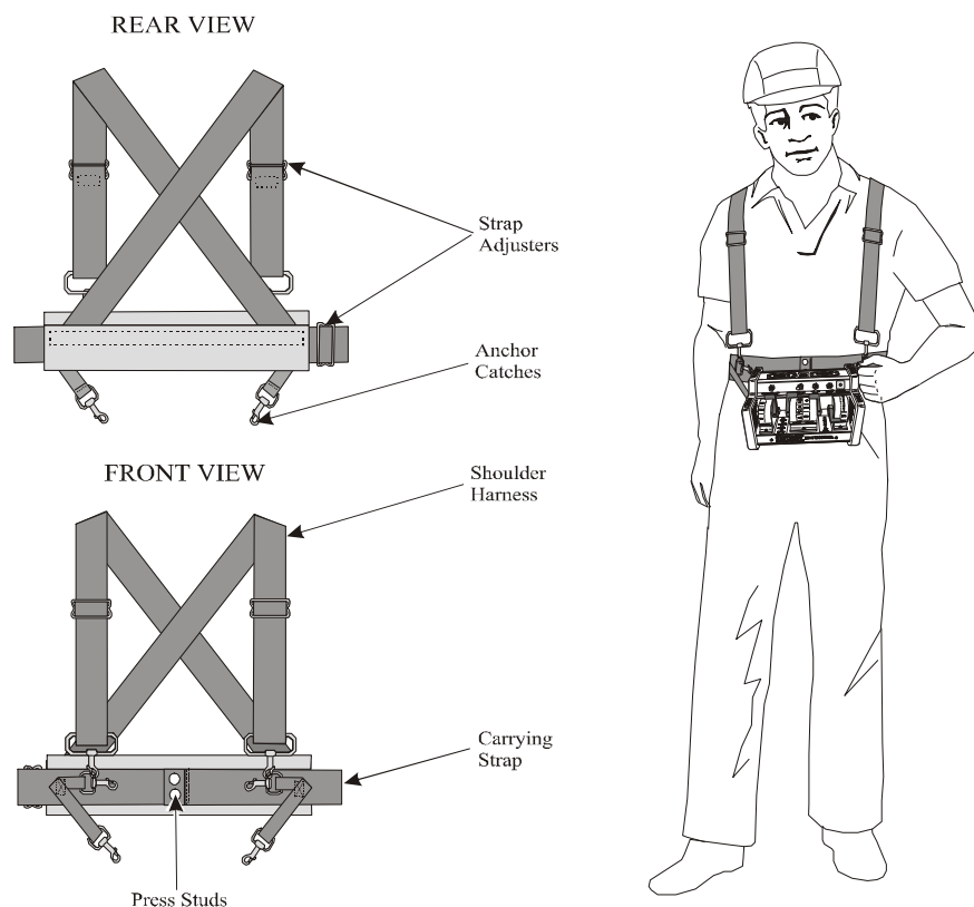
Figure 3-2. Standard carrying harness
