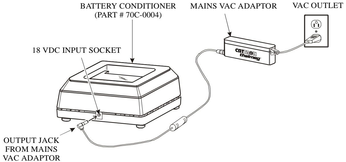
Figure 3-8. Ni -Cad Battery Pack Conditioning – interconnection details.
