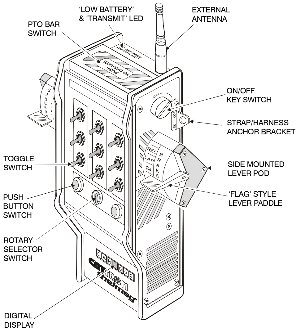
Figure 3-1. Toggle Controller – controls, indicators and features
