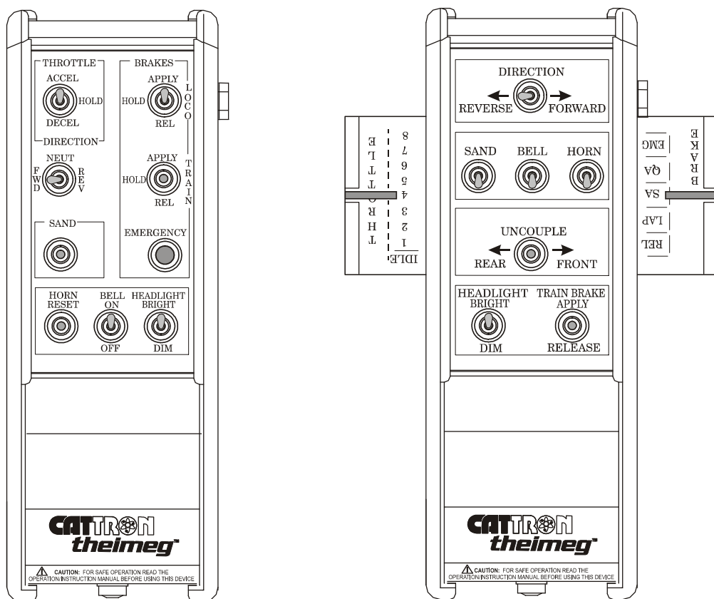
Figure 3-4. Locomotive Toggle Controller – typical configurations
