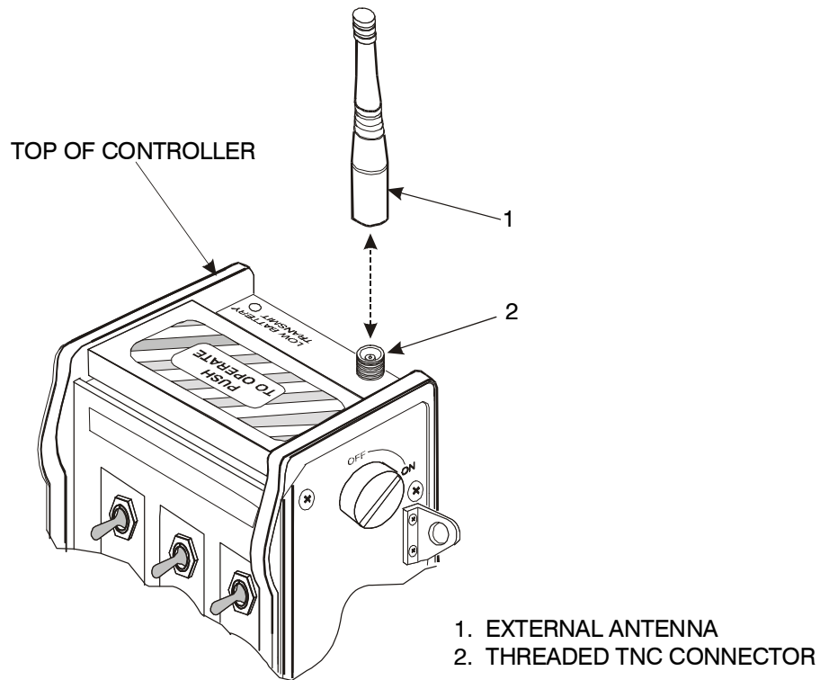
Figure 4-5. External Antenna Replacement.
