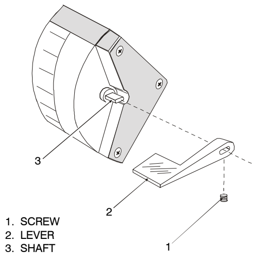
Figure 4-4. Lever Replacement.
