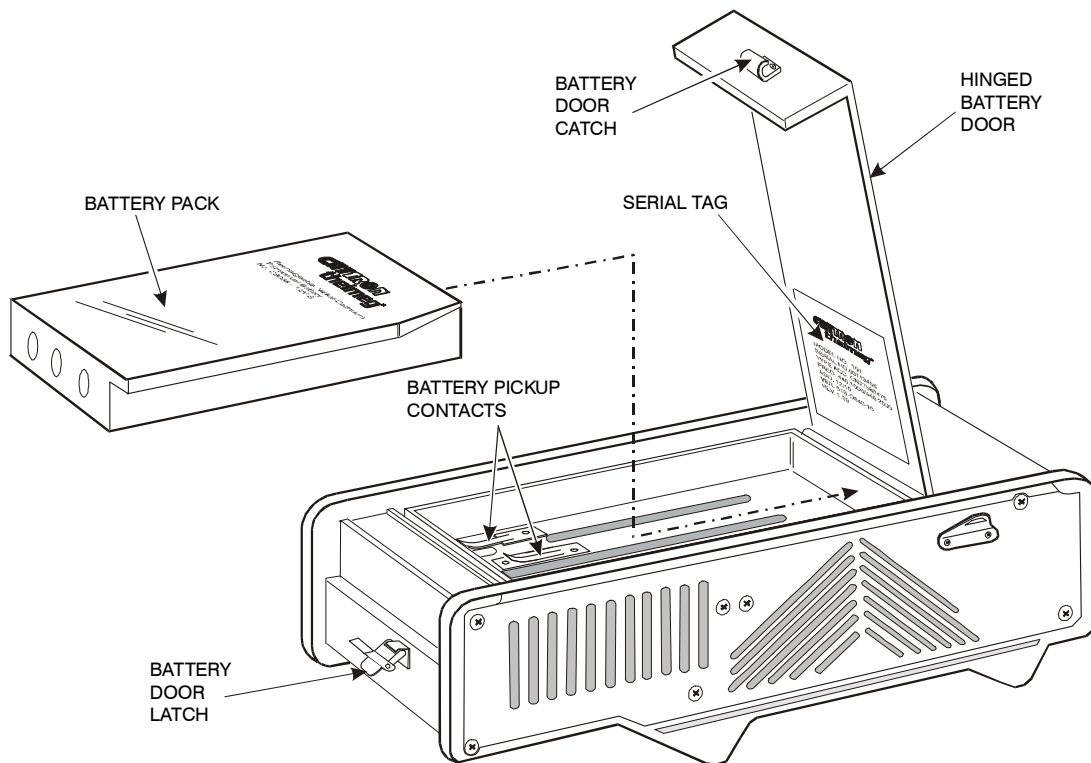
Figure 4-1. Battery Pack Replacement.
