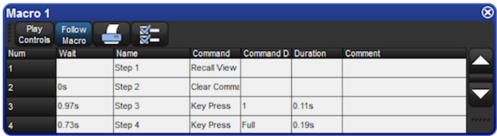
Figure 24.1. The Macro Window
