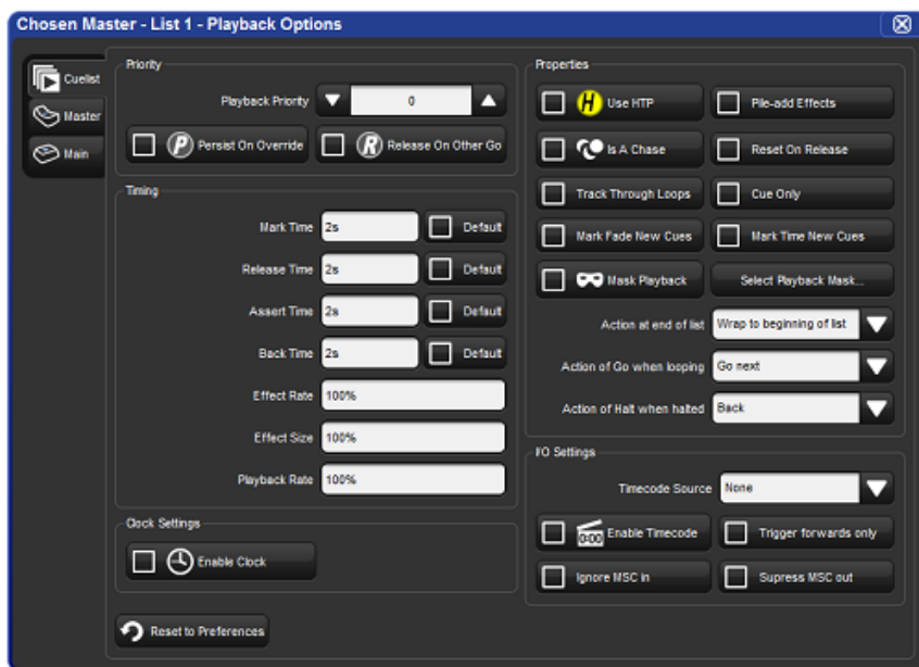
Figure 17.4. The Cuelist Pane of the Playback Options Window
