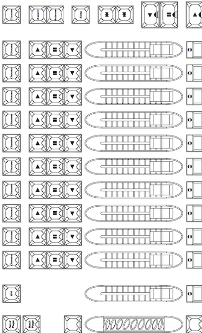
Figure 32.3. Playback section of the Hog 4 front panel
