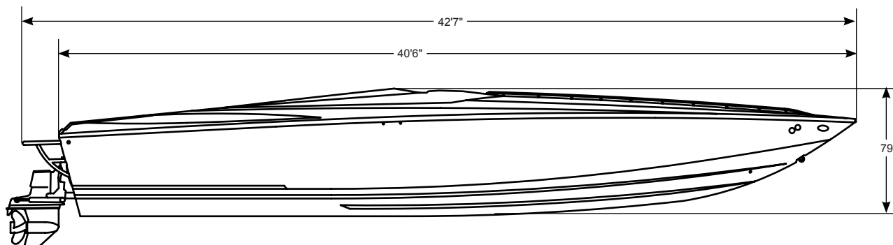
BOAT DIMENSIONS AND CLEARANCES (FIG. 2.2.1)
