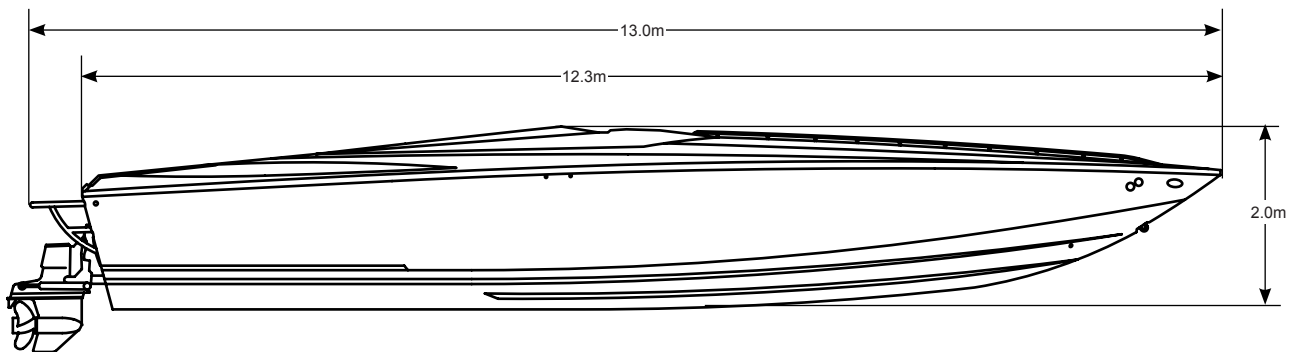
BOAT DIMENSIONS AND CLEARANCES (FIG. 2.3.1)
