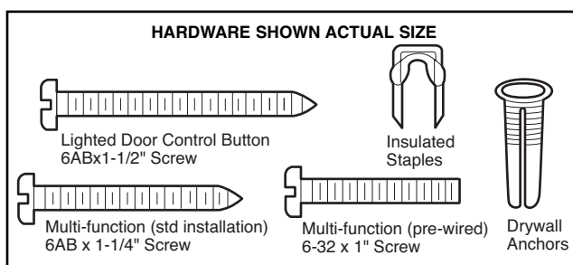
Figure 1 STANDARD INSTALLATION
