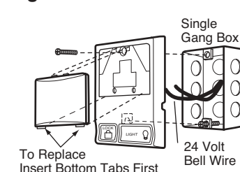
Figure 4 REMOVE COVER
