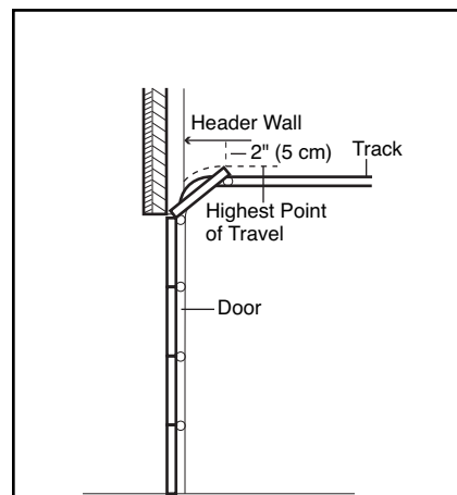
Sectional door with curved track
