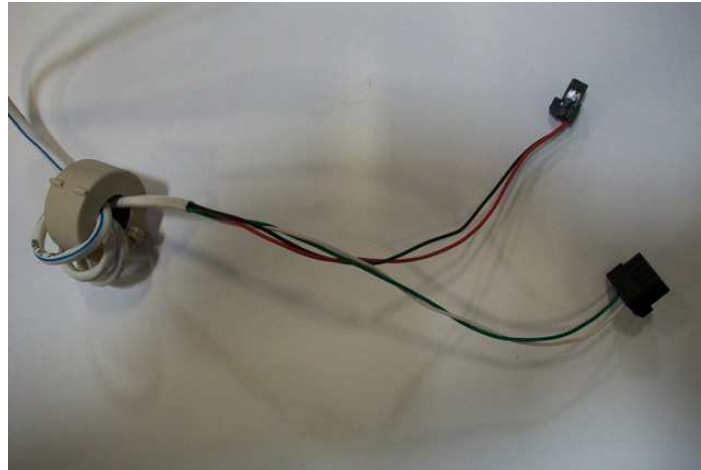
Figure 8 SSB Light/Sounder cable with ferrite core.
