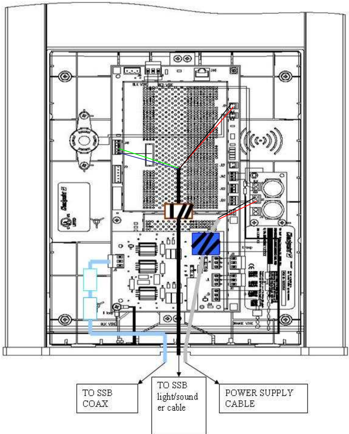
Figure 15 Classic Street PSB Antenna Wiring
