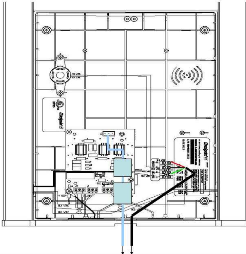
Figure 13 Classic Street SSB Antenna Wiring
