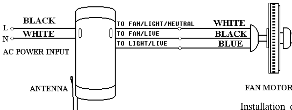
Ceiling Fan Remote Control Wiring Connection
