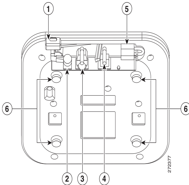
Figure 3 Access Point Ports and Connections (bottom)-AIR2602E and 2602I Models
