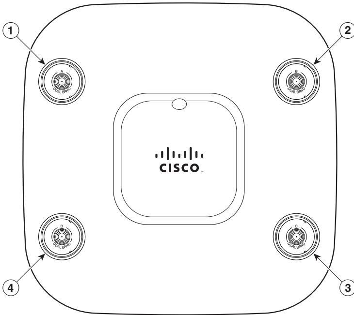
Figure 1 Access Point Ports and Connections (top)—3601E and 3602E Models
