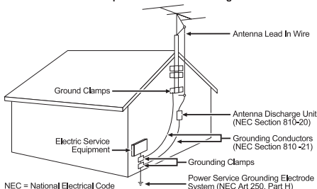
Example Of Antenna Grounding
