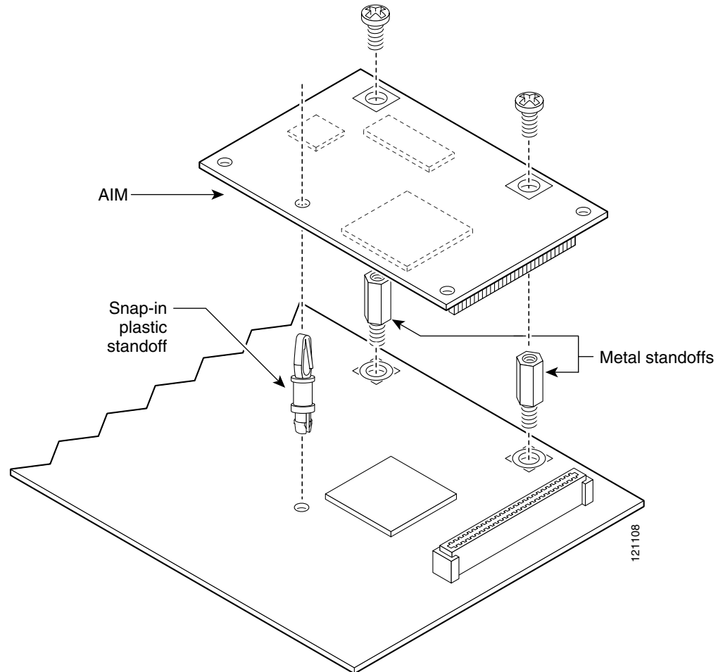
Figure 8-9 Connecting the AIM to the System Board
