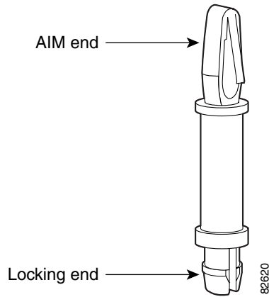
Figure 8-8 Plastic Standoff Orientation
