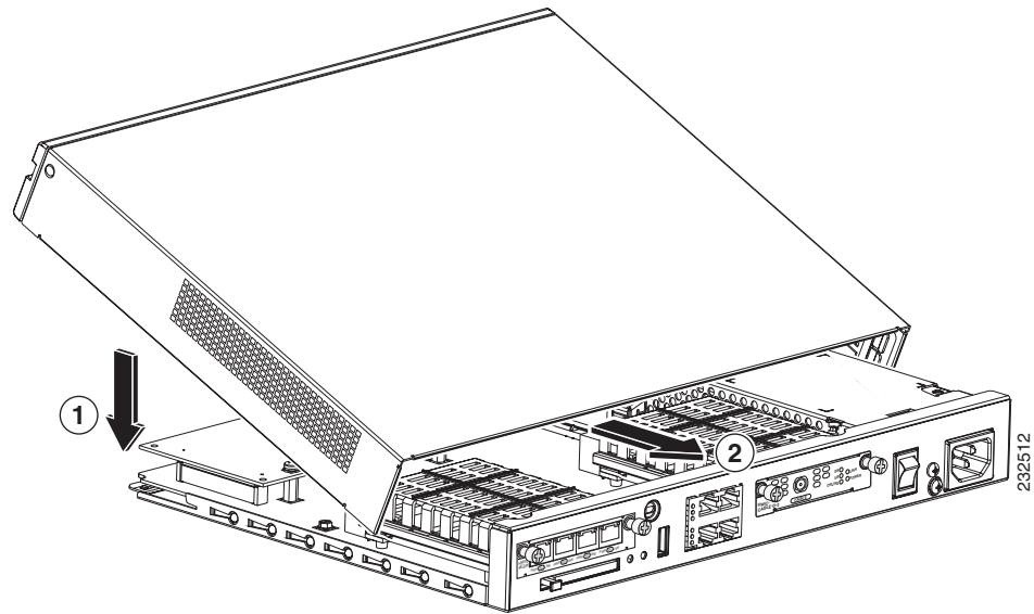
Figure 8-11 Closing the Chassis
