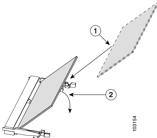
Figure 8-6 Installing a SODIMM
