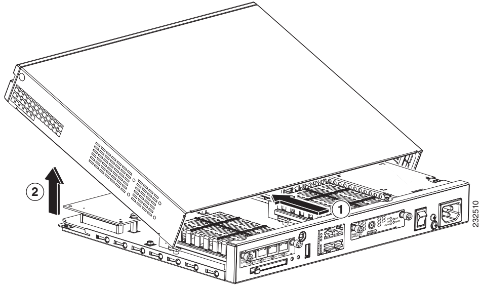
Figure 8-3 Removing the Cover of the Cisco 1805 Router
