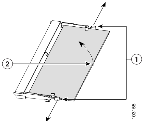
Figure 8-5 Removing a SODIMM
