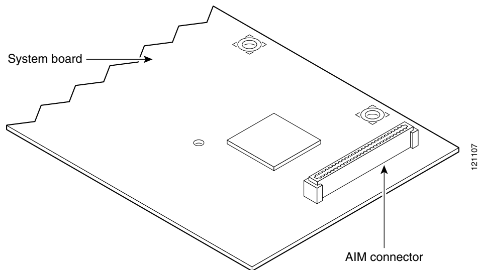
Figure 8-7 Location of Metal Standoff Attachment Locations
