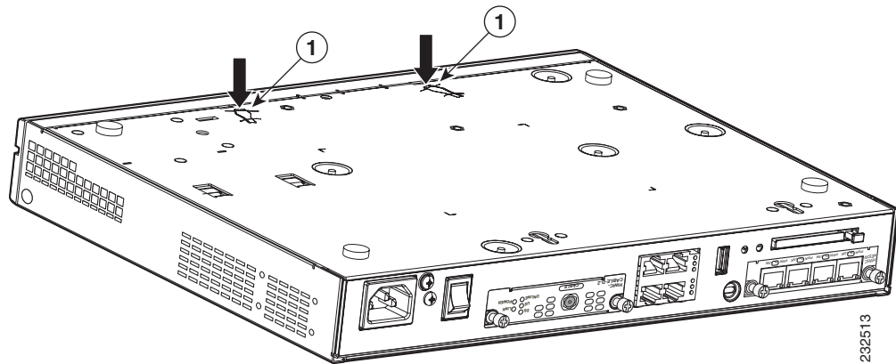
Figure 8-2 Screwdriver Pry Points
