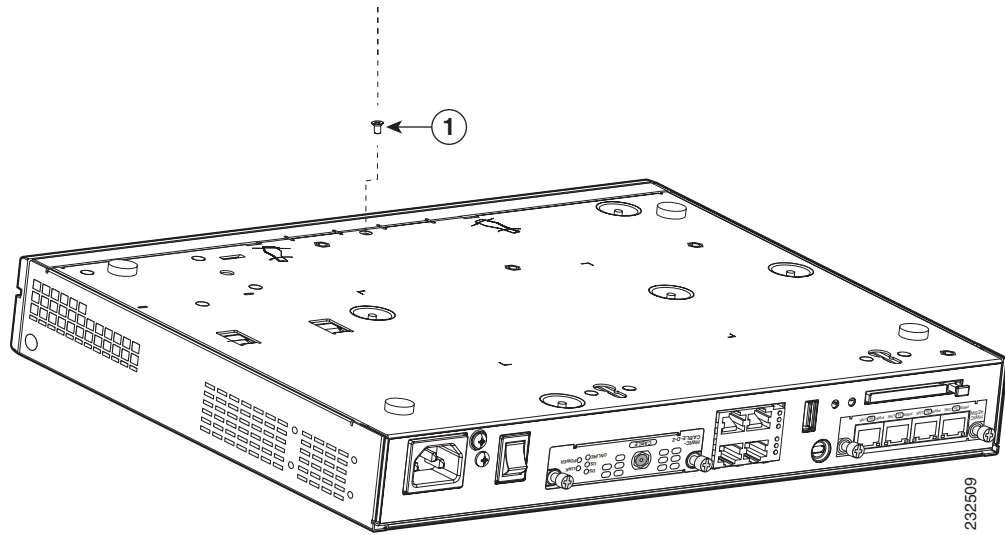
Figure 8-1 Removing the Chassis Screw
