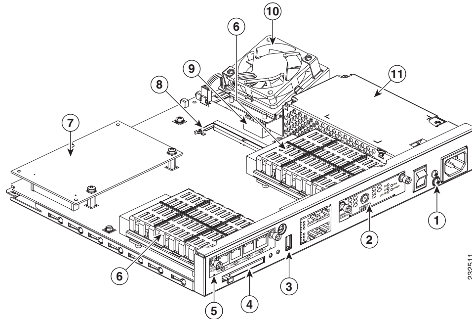
Figure 8-4 Cisco 1805 Cable Router (Internal View)
