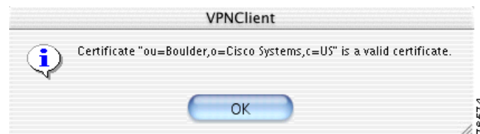
Figure 6-12 Verify Certificate
