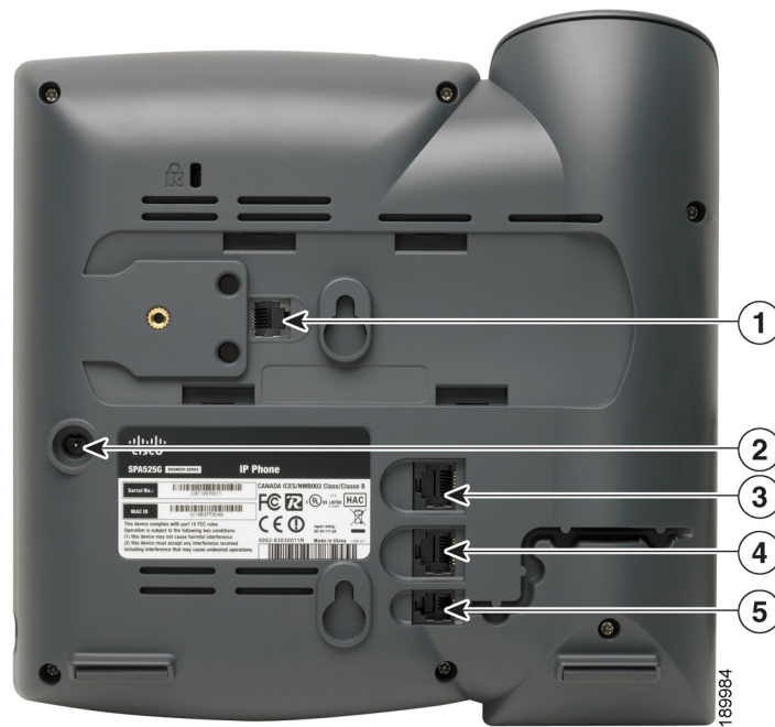
Figure 2 Cisco SPA525G and SPA525G2 IP Phone Connections
