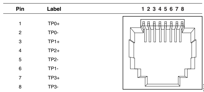
Figure A-1 10/100/1000 Port Pinouts
