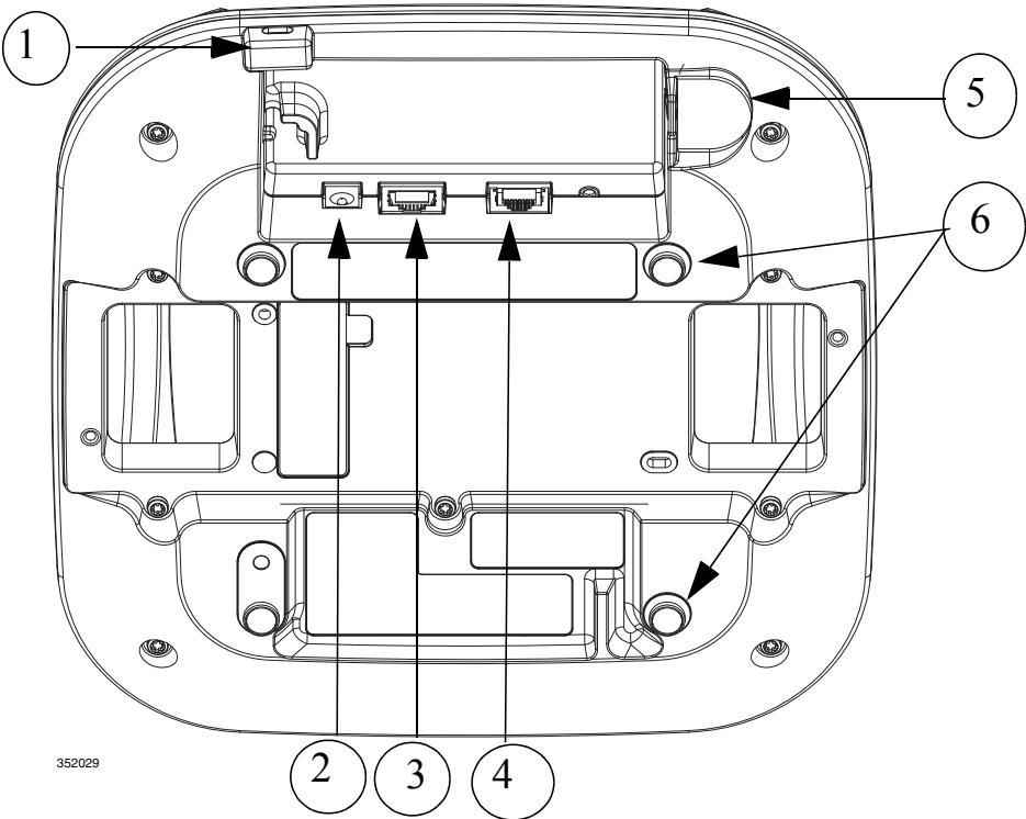
Figure 3 Access Point Ports and Connections (bottom)-AIR3702E and 3702I Models
