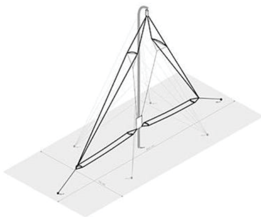
Figure 2-28: Complex Antenna
