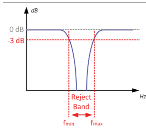
Figure 2-38: Band Reject Filters
