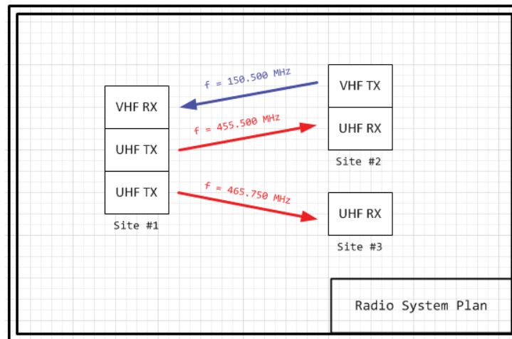
Figure 3-1: Communications Plan
