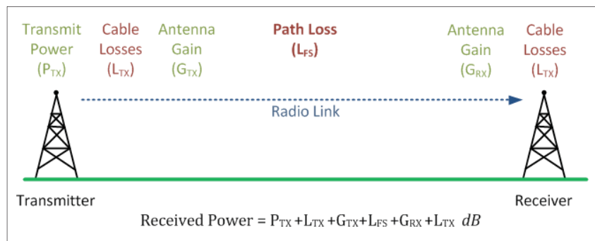
Figure 3-2: Link Budget Diagram
