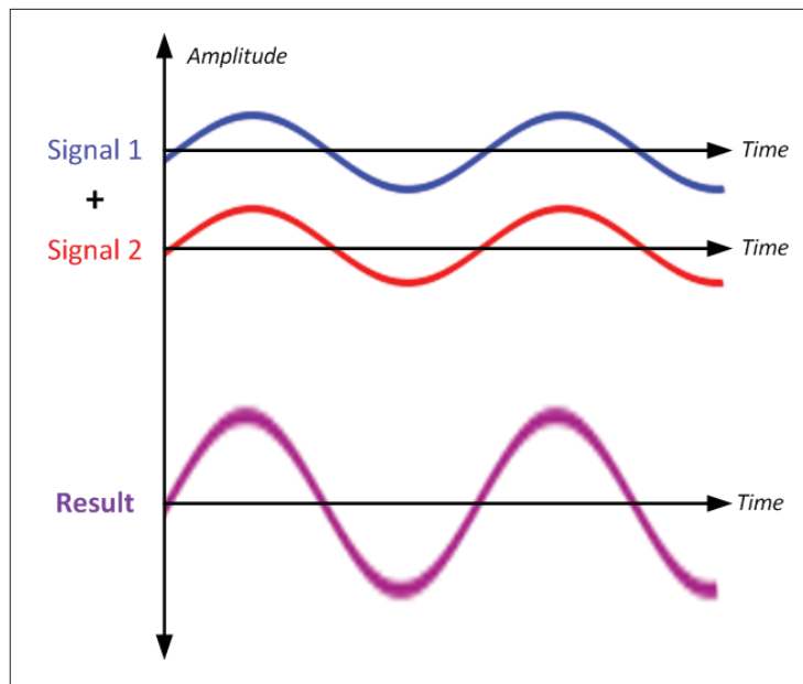
Figure 2-34: In-Phase Signals
