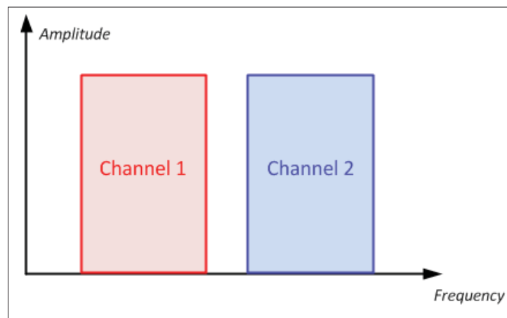
Figure 3-8: FDMA Concept
