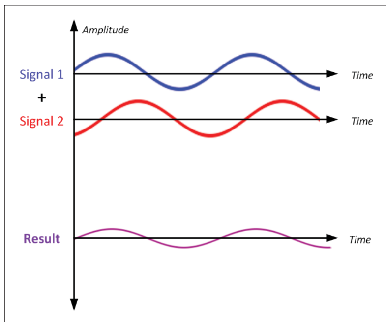
Figure 2-35: Out-of-Phase Signals
