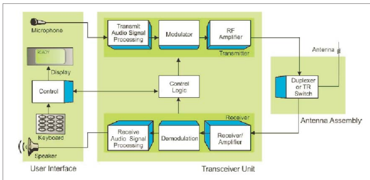
Figure 3-5: Transceiver Equipment
