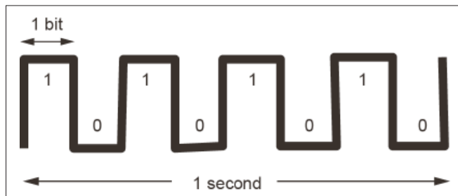
Figure 2-13: Bitrate
