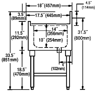
side view dimensions of all 1800 Series underbar sinks
