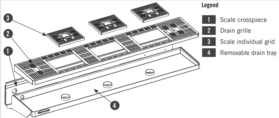
Fig. 5 - Precision scale - 2 and 3 brewing groups
