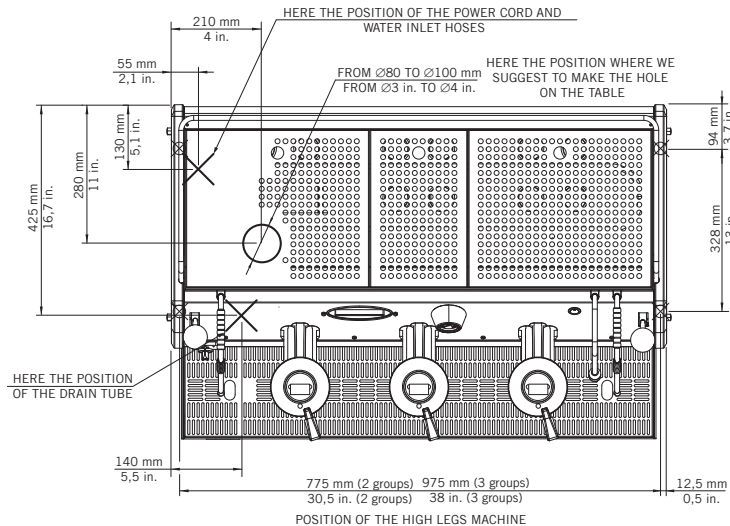
Fig. 2 - Installation guide
