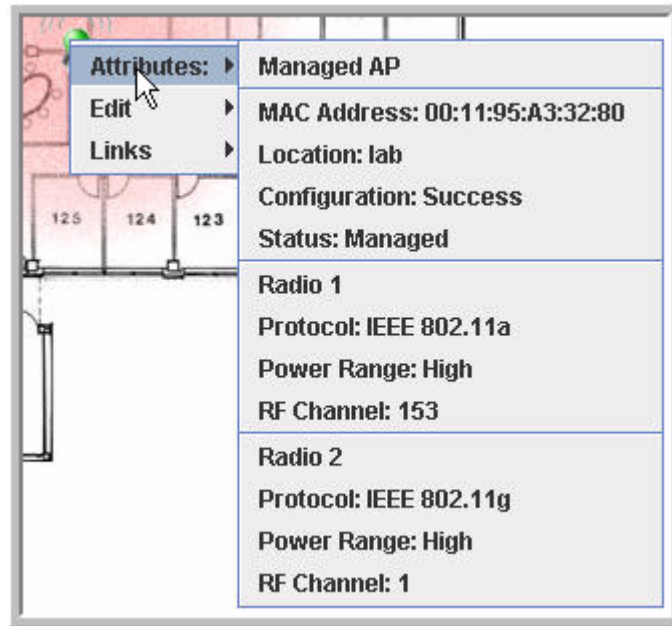
Figure 82. Wireless Component Attributes
