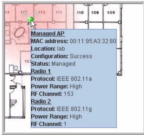
Figure 81. Tool Tip for Radio Managed AP Information
