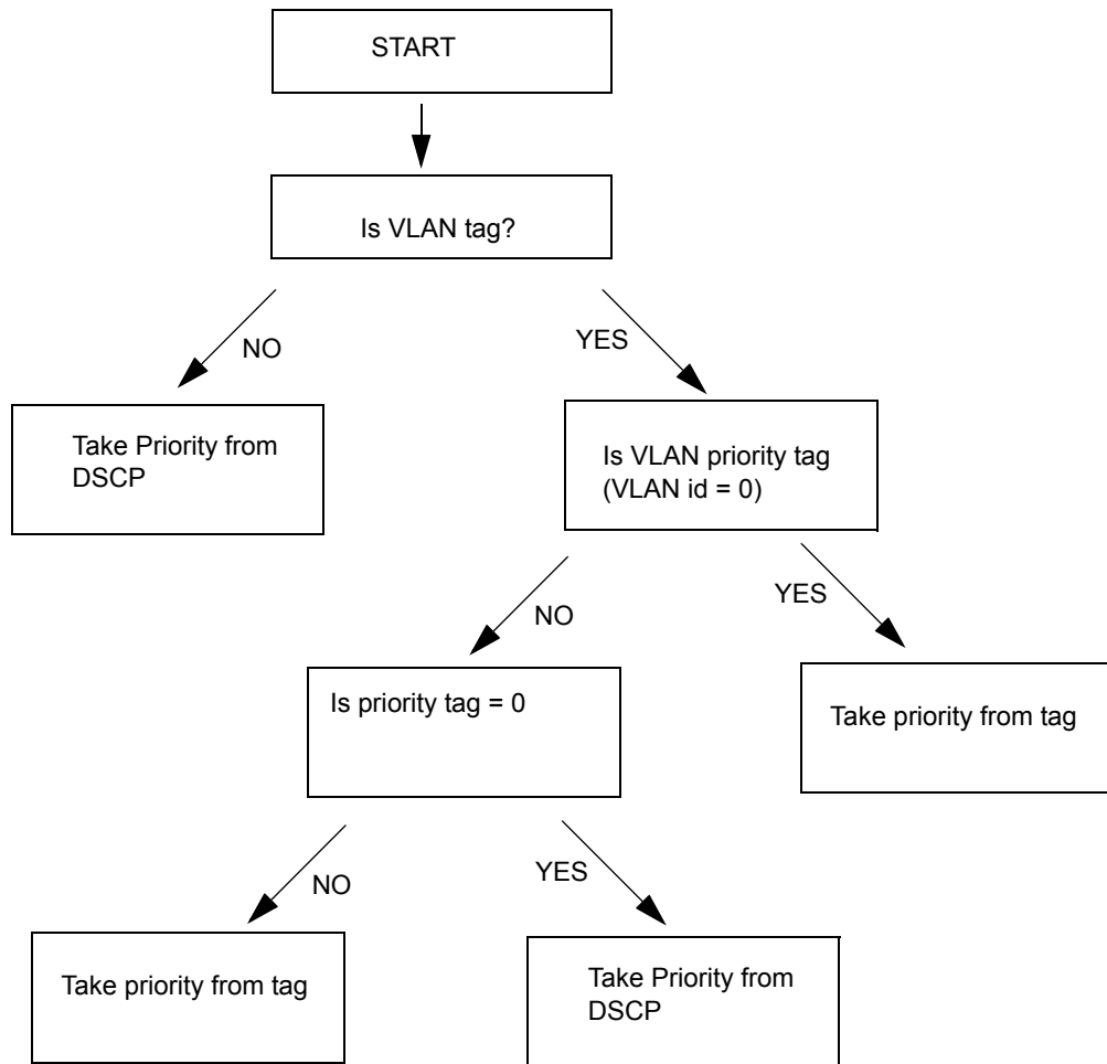
Figure 84. Traffic Prioritization
