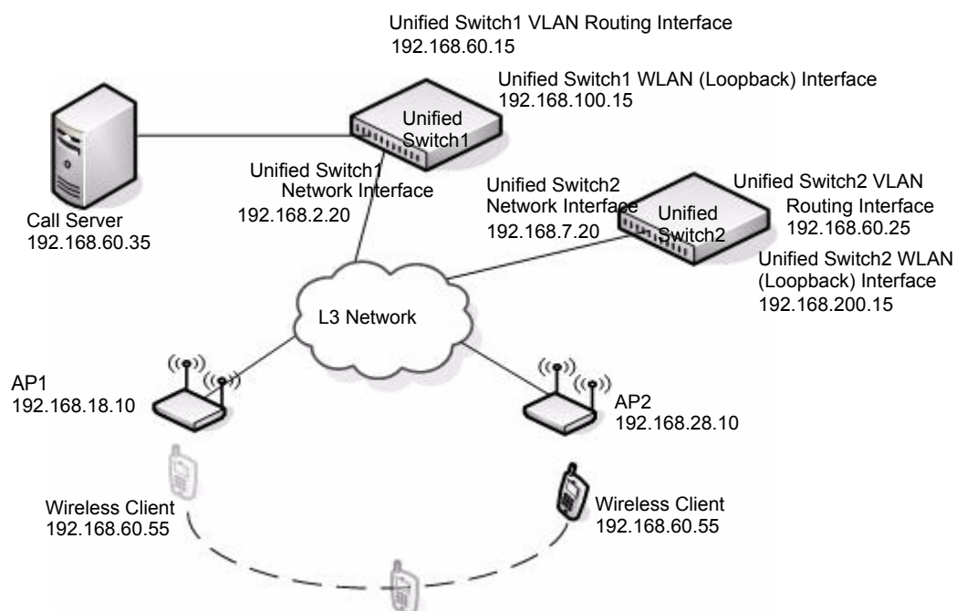
Figure 83. Example of a Network with L3 Tunnel Subnet
