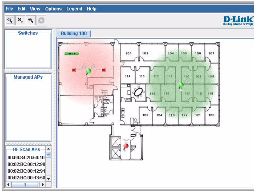
Figure 73. Sample WLAN Visualization
