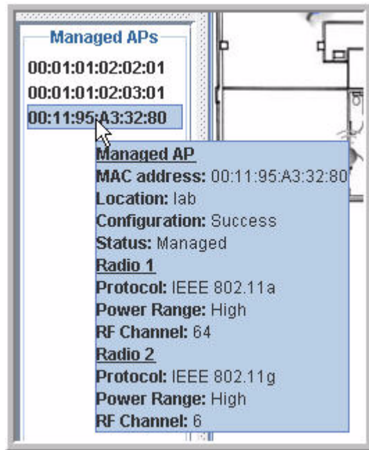
Figure 76. Component Tool Tip
