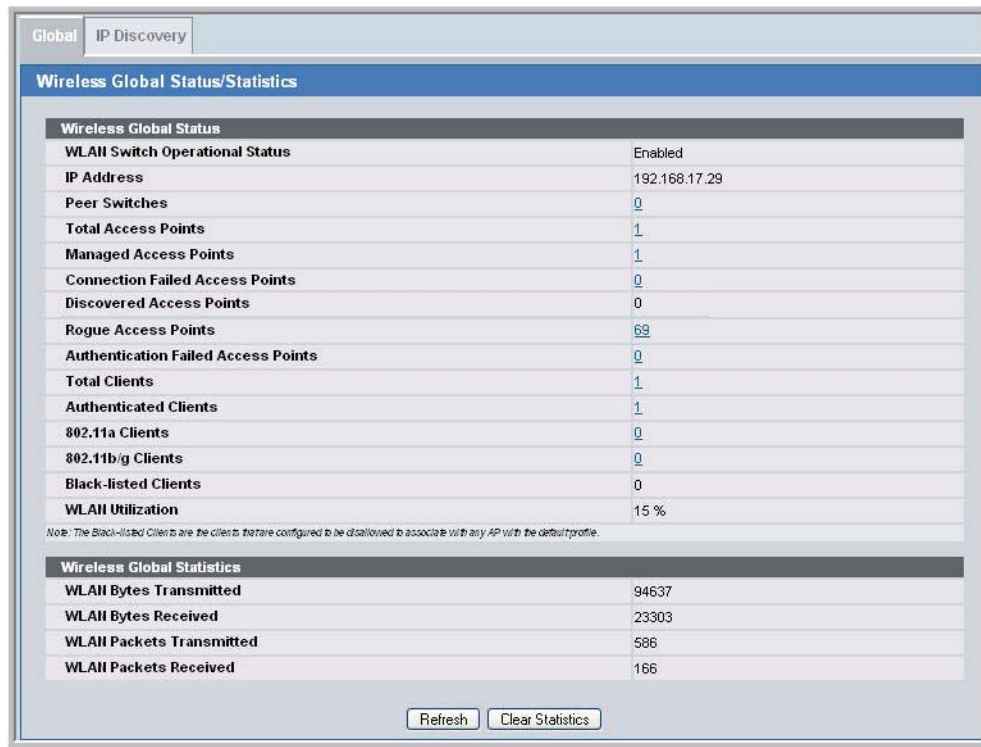
Figure 55. Global WLAN Status
