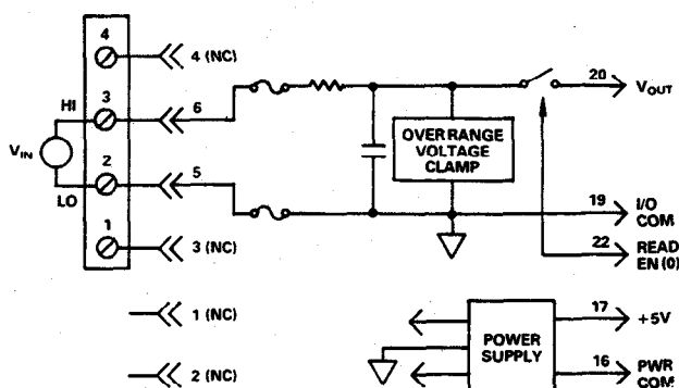
Figure 2.11. AC1367 Functional Block Diagram
