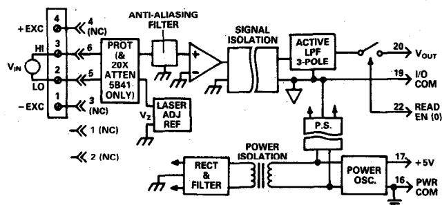
Figure 2.8. 5B40 and 5B41 Functional Block Diagram
