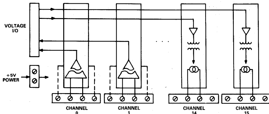
Figure 3.1. 5B01 Diagram
