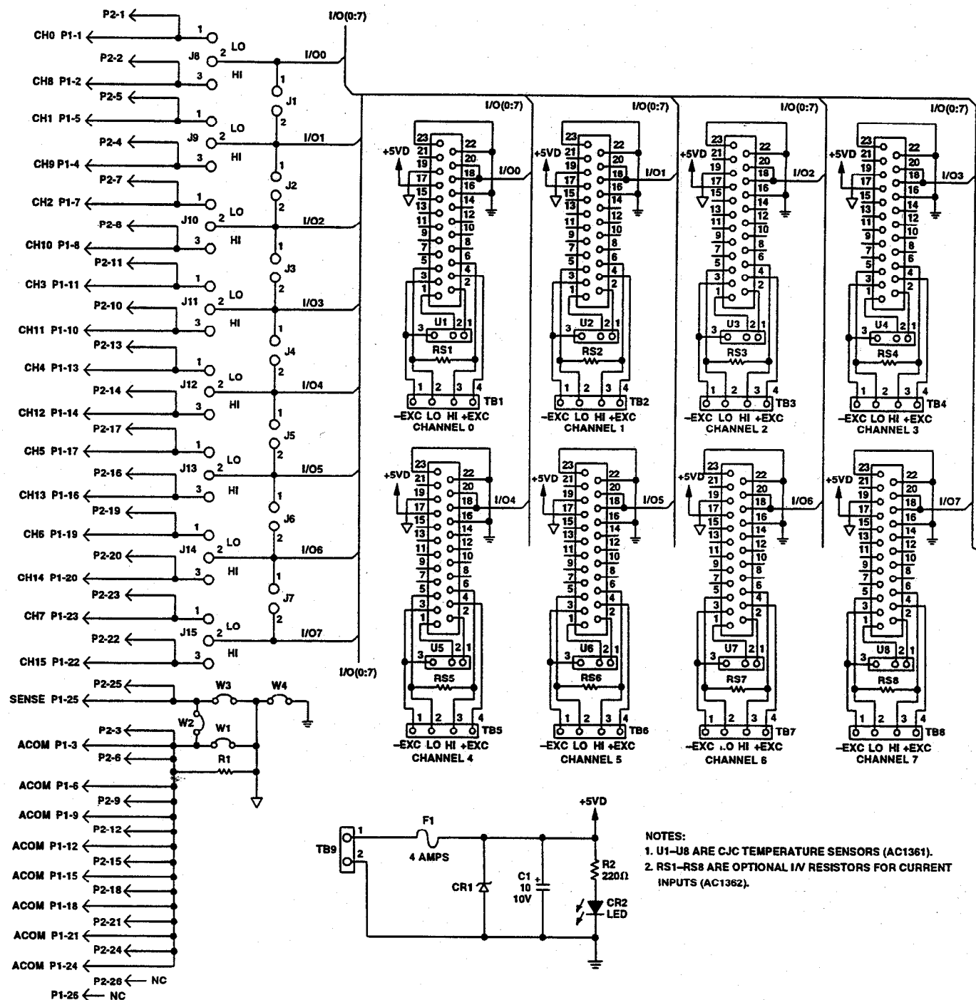
Figure 5. 5B08 Schematic Diagram
