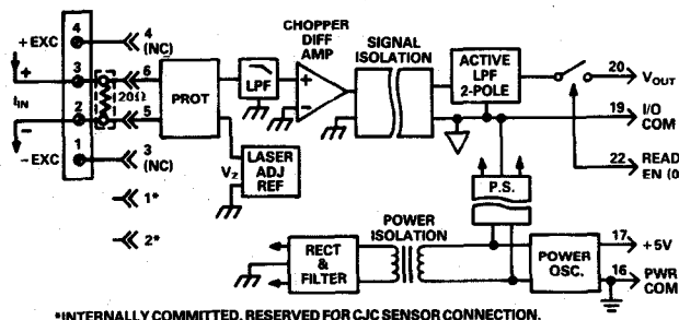
Figure 2.3. 5B32 Functional Block Diagram
