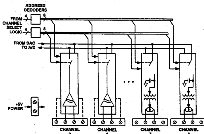
Figure 3. 5B08-MUX Functional Block Diagram
