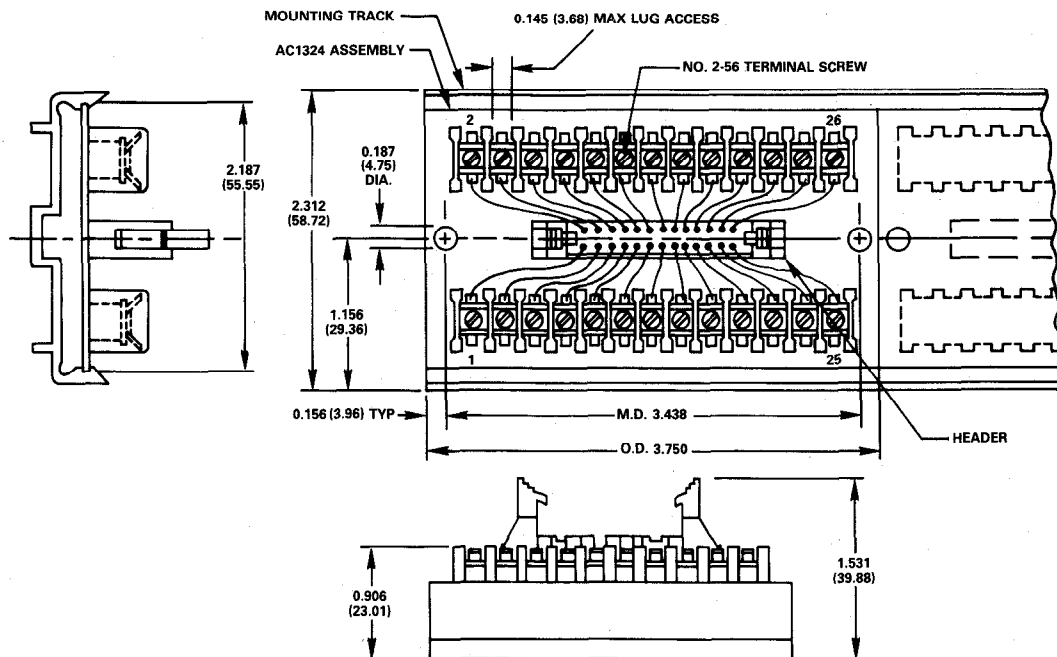
Figure 3.15. AC1324 Diagram (dimensions in inches and (mm))
