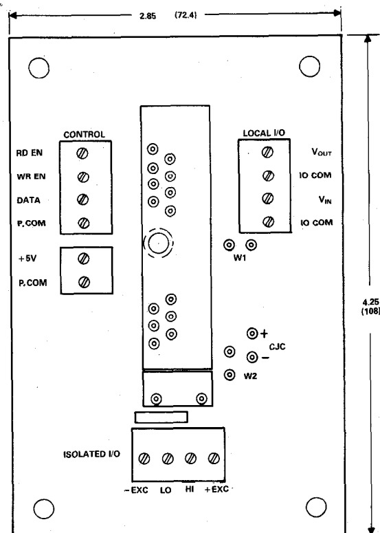
Figure 4.7. AC1360.
