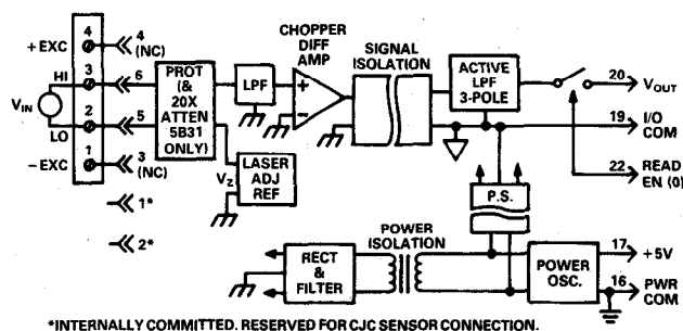
Figure 2.2. 5B30 and 5B31 Functional Block Diagram
