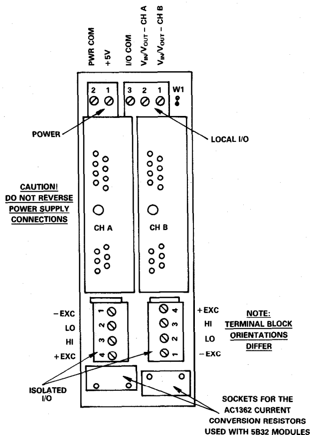
Figure 3.9. 5B04 Wiring
