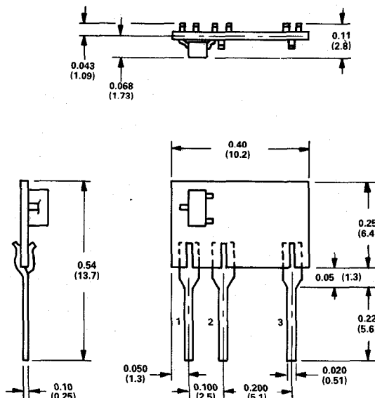
Figure 4.4. AC1361 Outline
