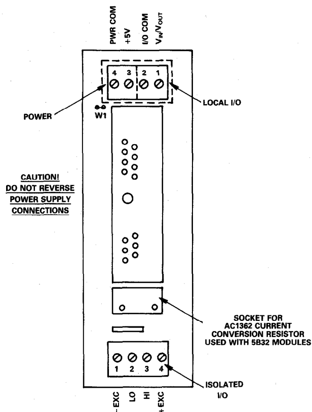
Figure 3.8. 5B03 Wiring Diagram
