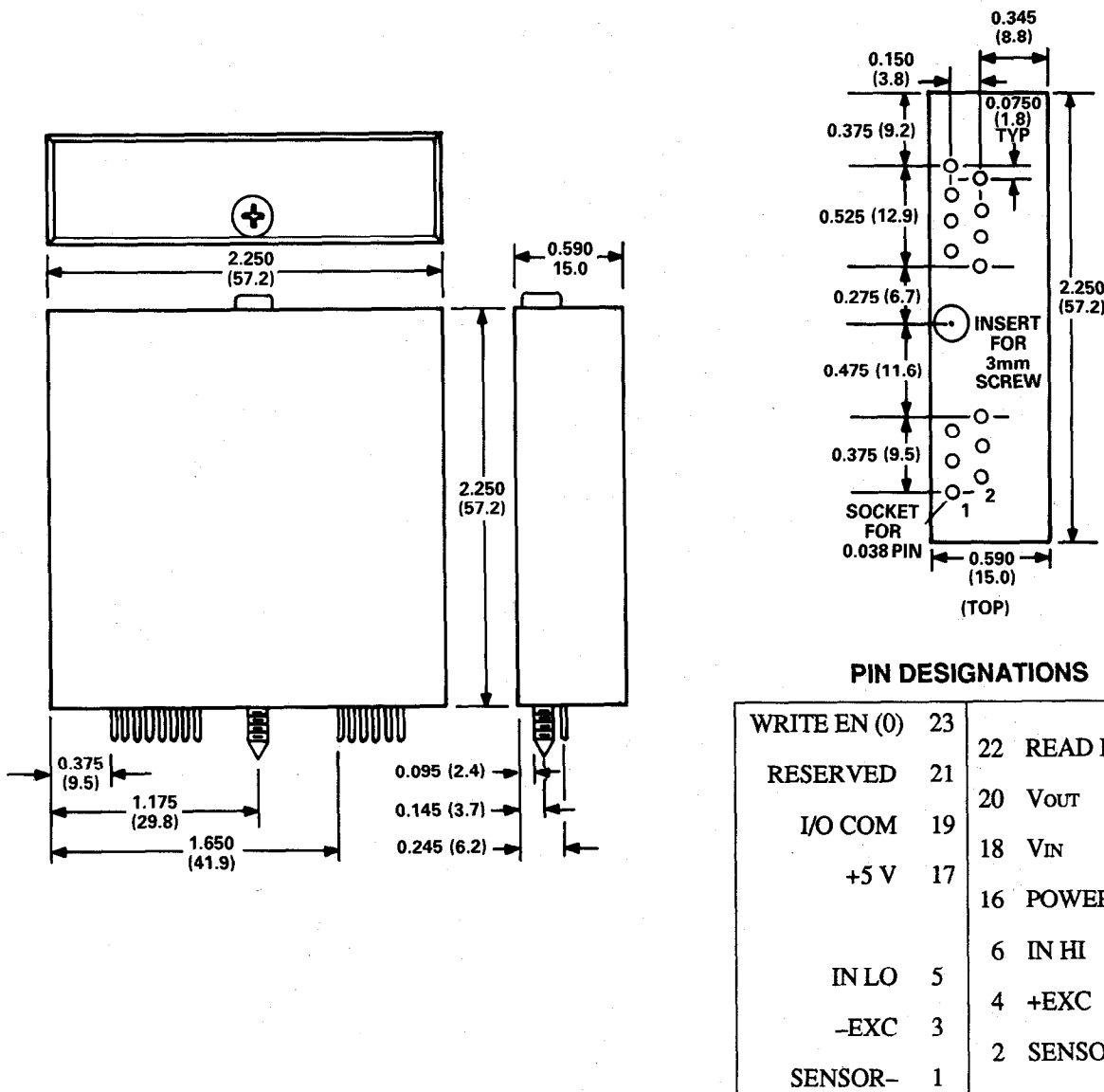
Figure 4.1. 5B Series Input Module Outline and Pin Designations
