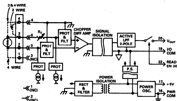
Figure 2.4. 5B34 Functional Block Diagram
