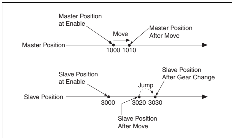
Figure 10-3. Absolute Gearing at Gear Ratio Change
