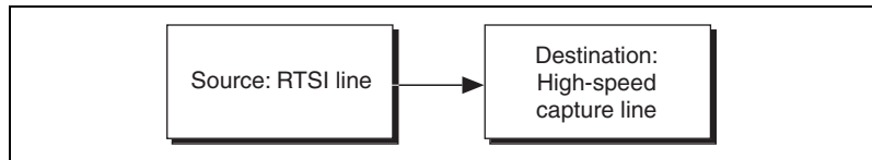
Figure 12-25. High-Speed Capture Input Using RTSI
