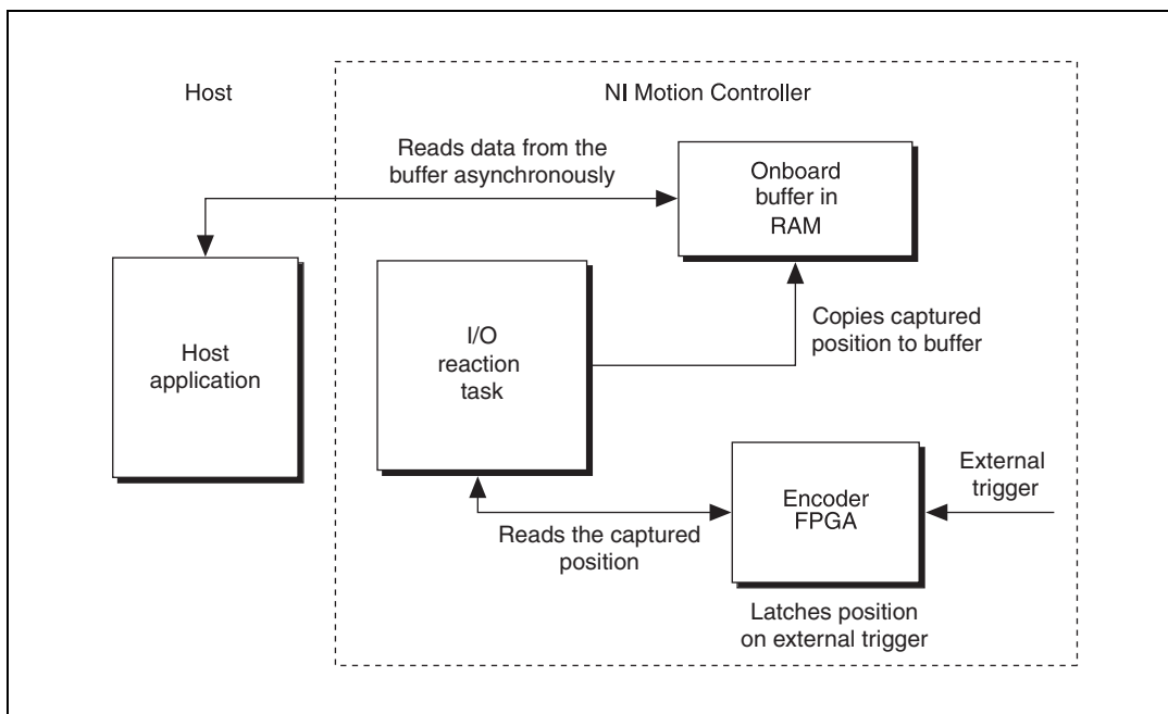
Figure 14-13. Onboard Buffer Data Flow
