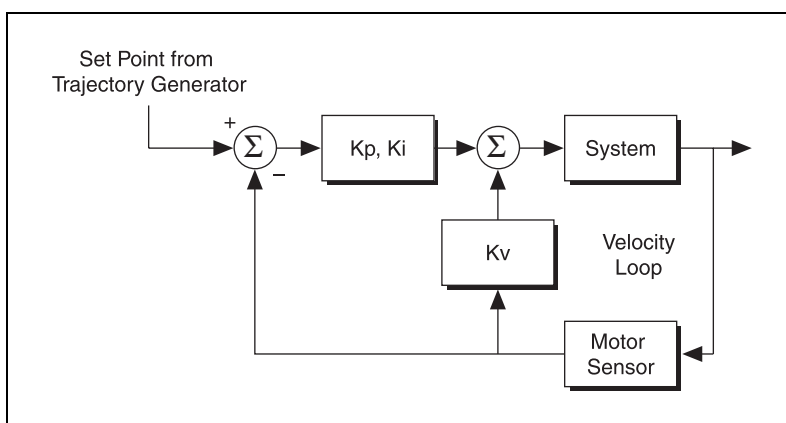
Figure 3-5. Velocity Feedback
