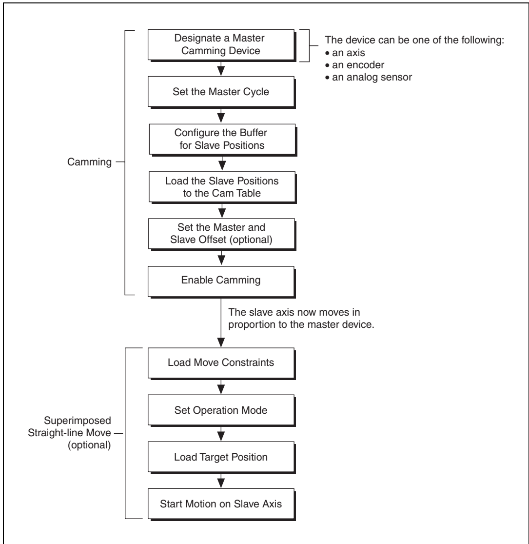
Figure 10-8. Camming Algorithm
