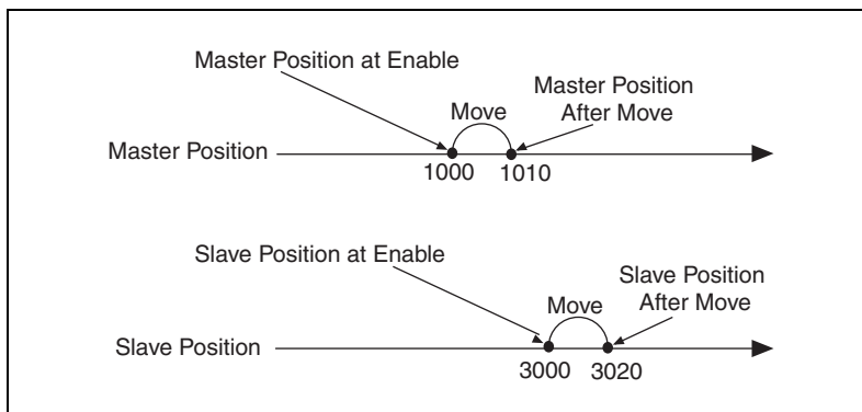
Figure 10-2. Relative Gearing at Enable
