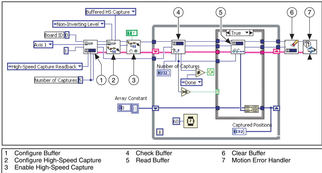
Figure 12-17. Buffered High-Speed Capture in LabVIEW
