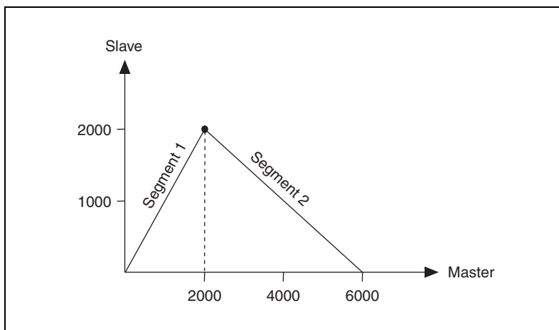
Figure 10-10. First and Second Move Segment Profile
