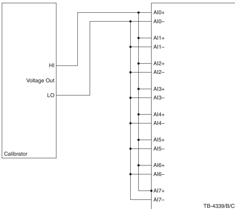
Figure 2. Calibrator to TB-4339/B/C Voltage and Ratio Mode Connections
