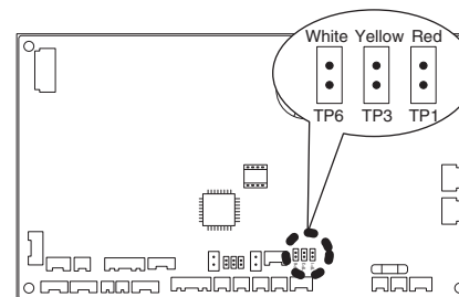
Indoor control board
