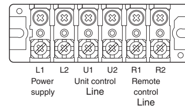
Y1, D1, T1, F1, M1, P1, R1 Types 6P terminal board
