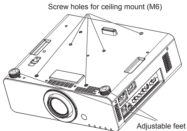
Fig. 1 The positions of screw holes for ceiling mount and adjustable feet
