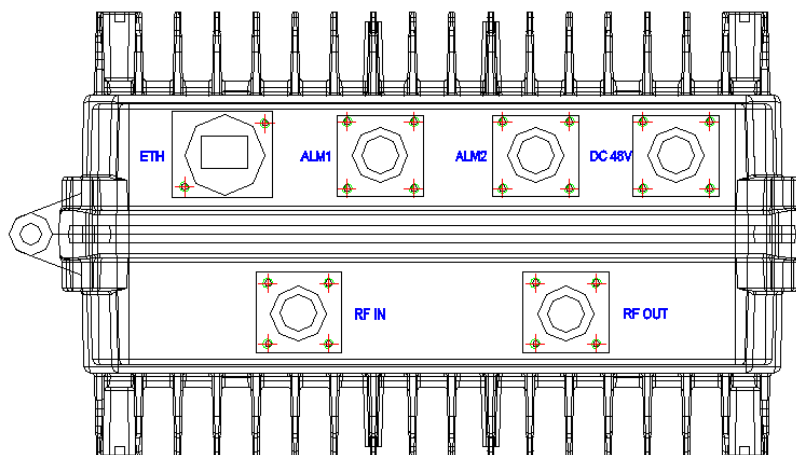
Figure 3: Equipment Connectors
