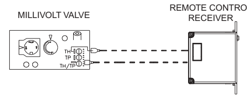
GENERIC WIRING DIAGRAM FOR RECEIVER. THE RECEIVER WIRE NEED TO CONNECT TO THE VALVE AT THE "TH" AND "TH/TP" JUNCTION
