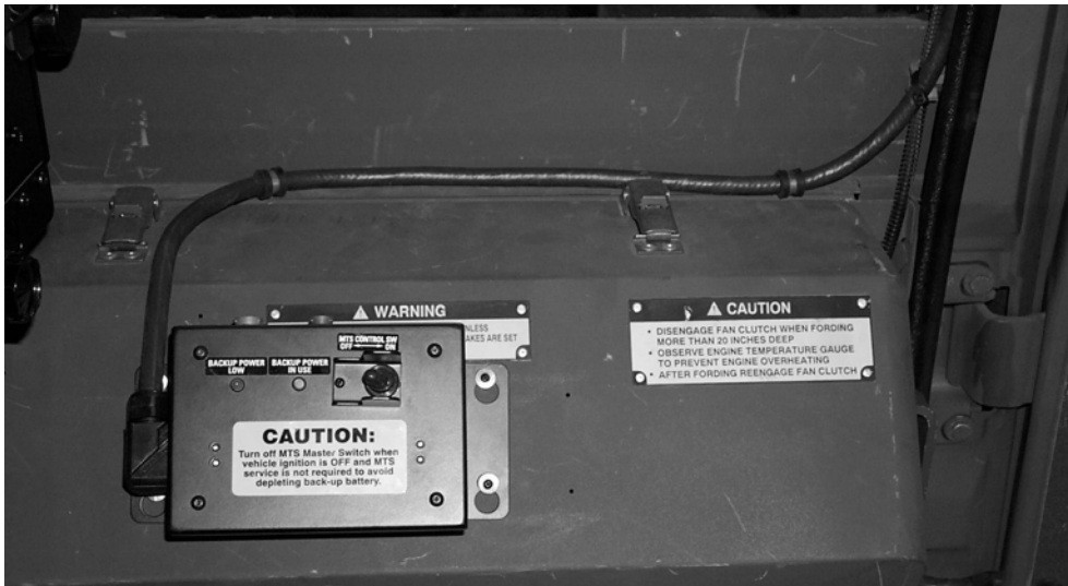
Figure 14-2 V2 Control Box mounted inside FMTV cab
