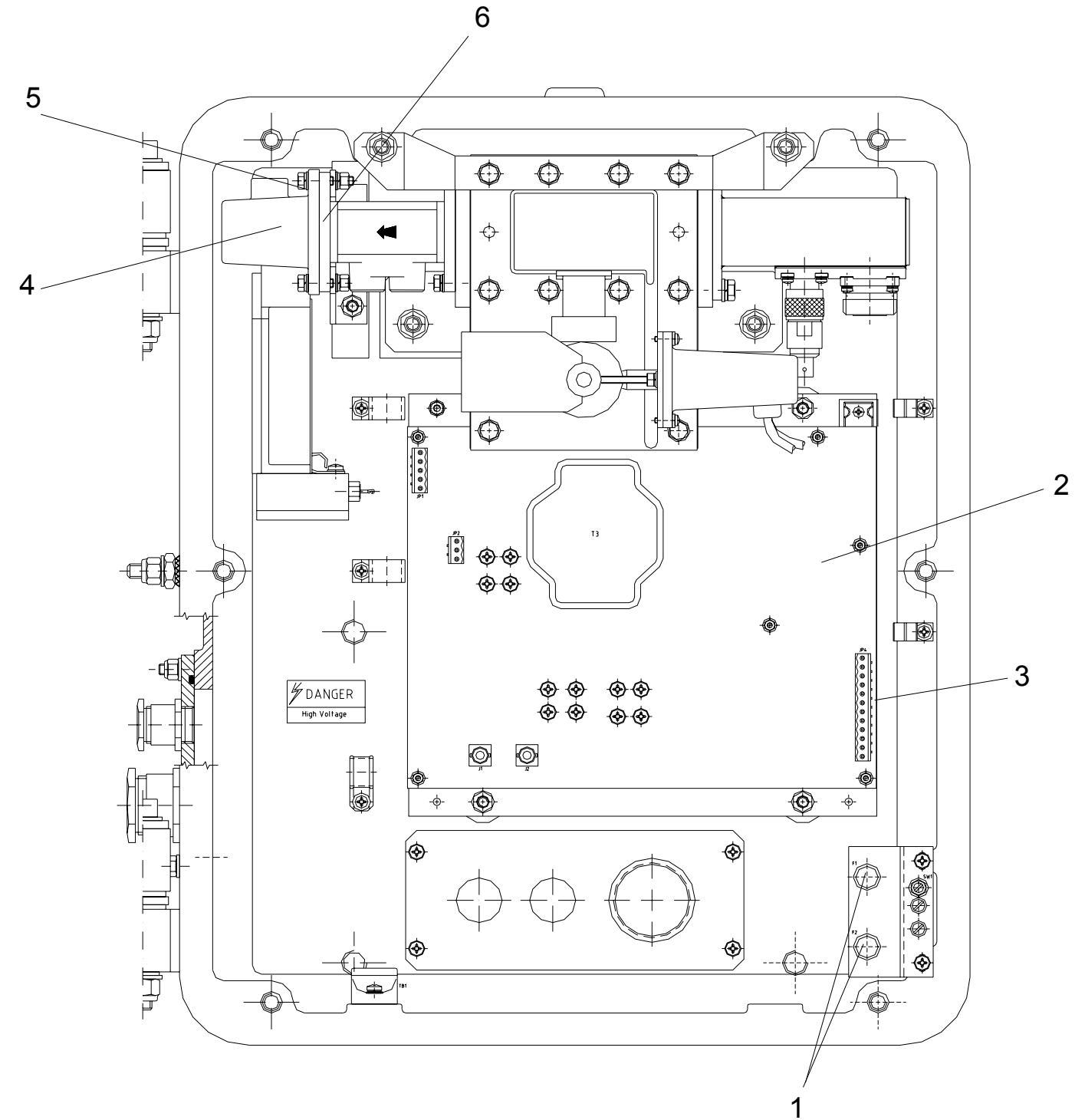
Figure 9.1.30 RTM 30S/U/D Unit - Internal View
