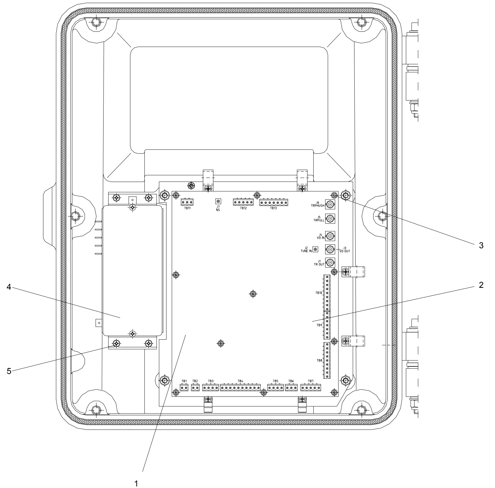
Figure 9.1.31 RTM 30S/U/D Unit - Internal View of the Cover
