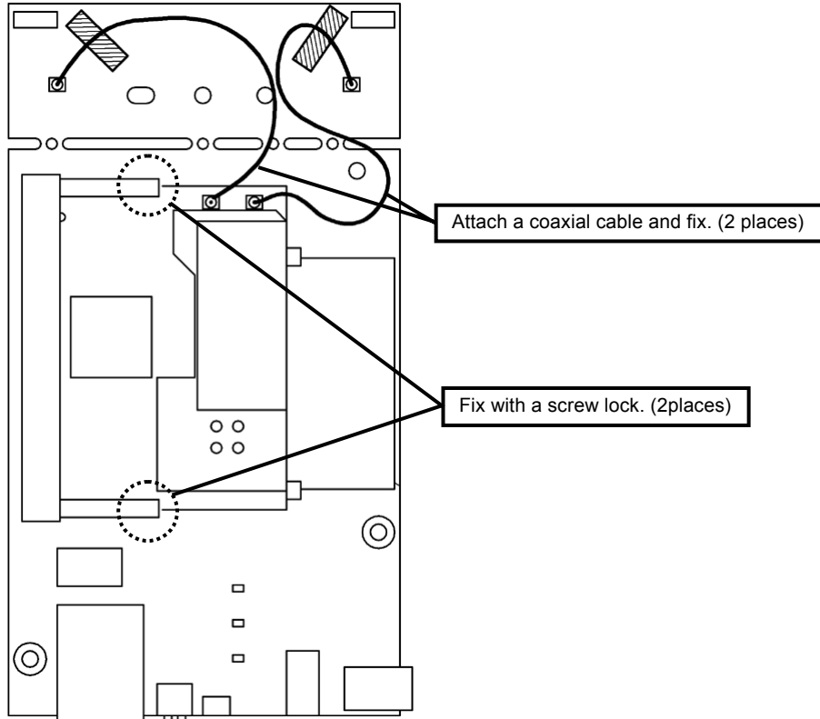
Figure2 : How to attach in FX-DS540-APDL-NR5
