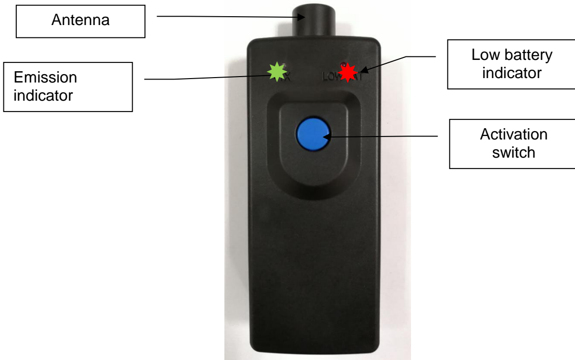
Front view
