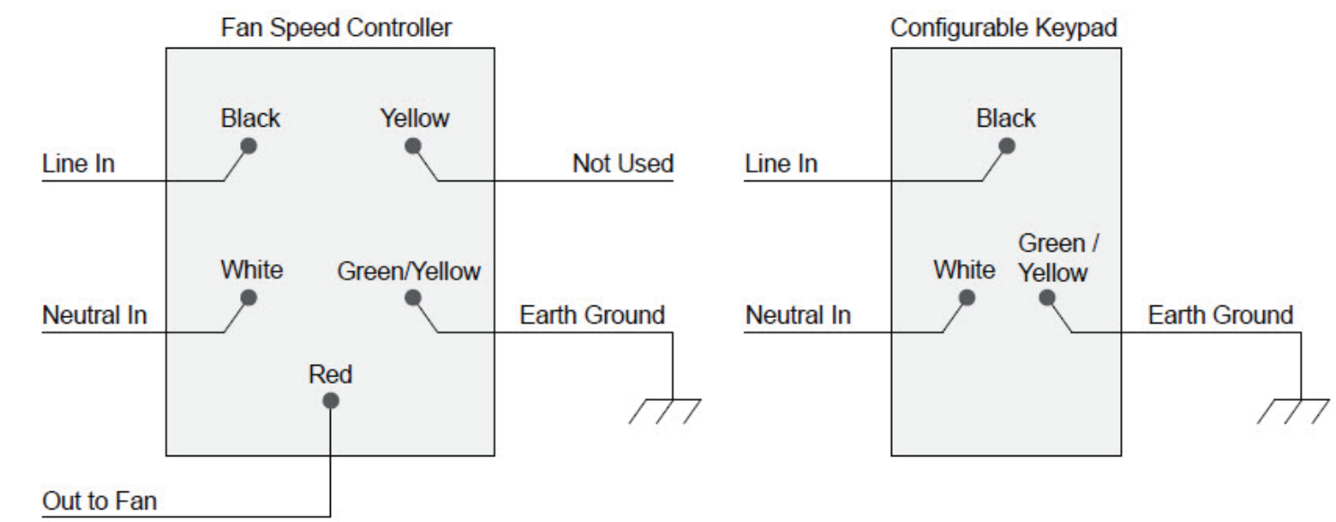
Figure 5. Multiple Device Location Using Configurable Keypad
