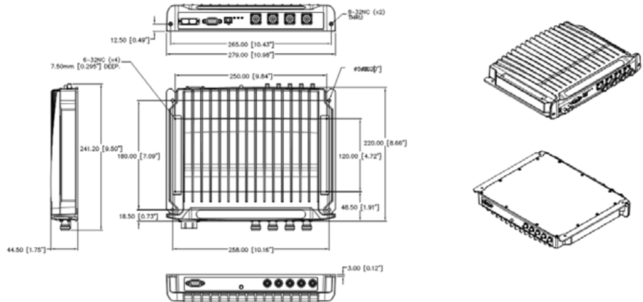
Figure 16: MA1000 RHU Dimensions
