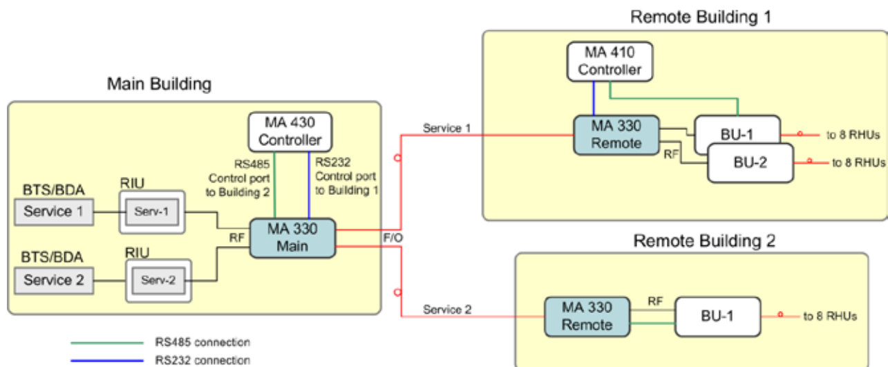
Figure 15: 330 System Installation Examples
