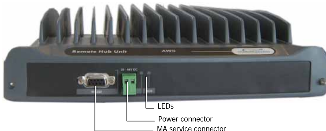
Figure 7. RHU Add-on Front panels
