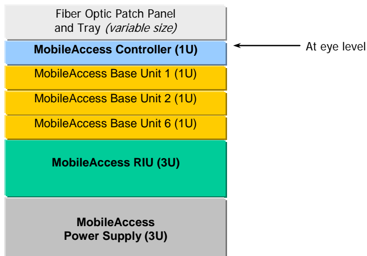
Figure 13: Recommended Order in the Communication Room Rack
