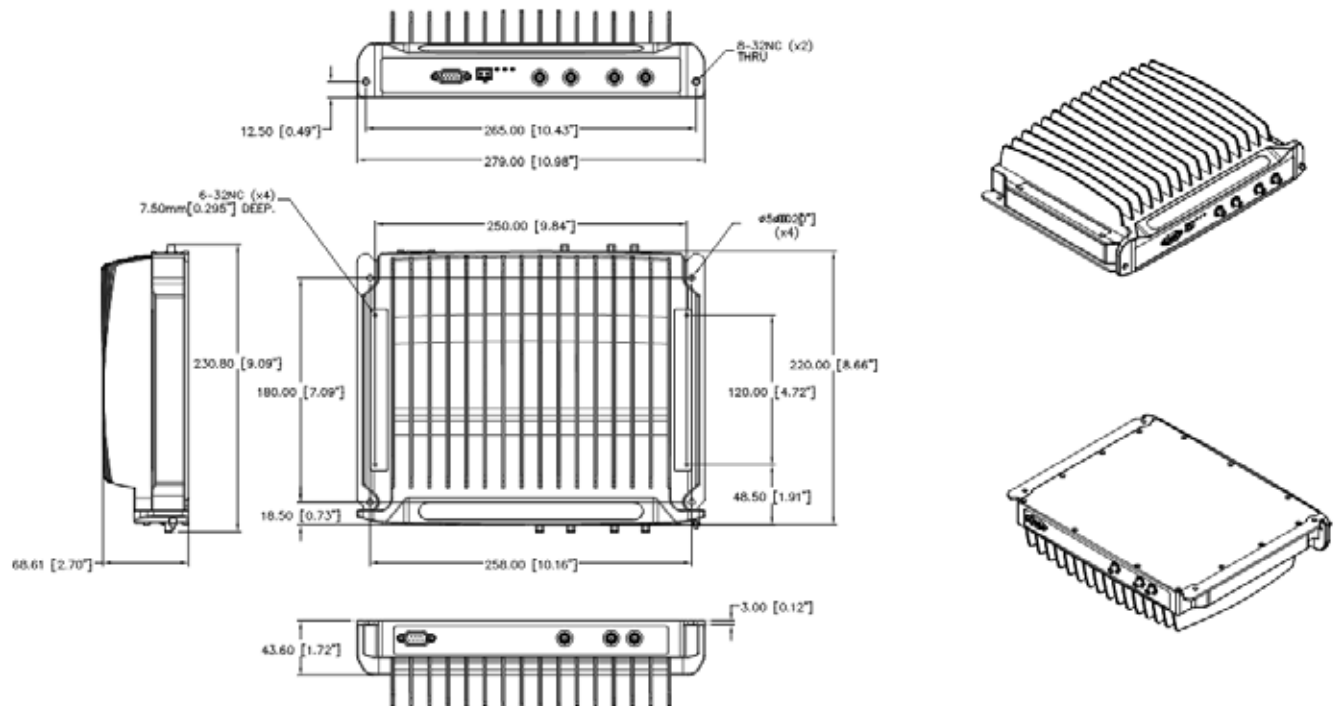
Figure 18. Add-On Dimensions
