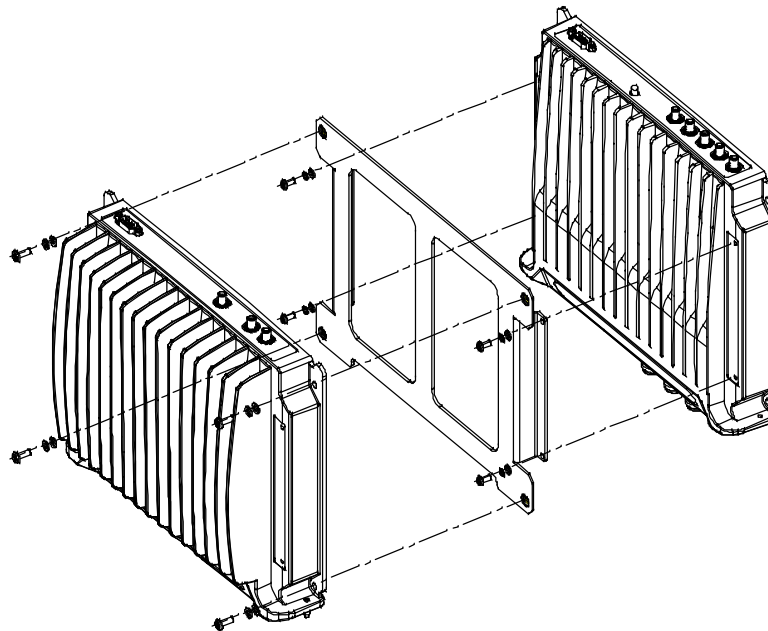
Figure 19. RHU Add-on to 1000 RHU Assembly
