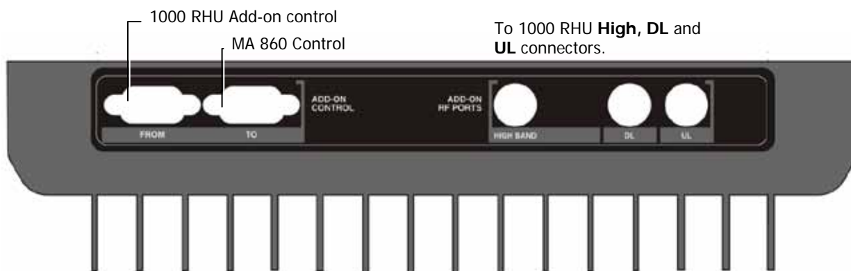
Figure 8. RHU Add-on Rear Panel
