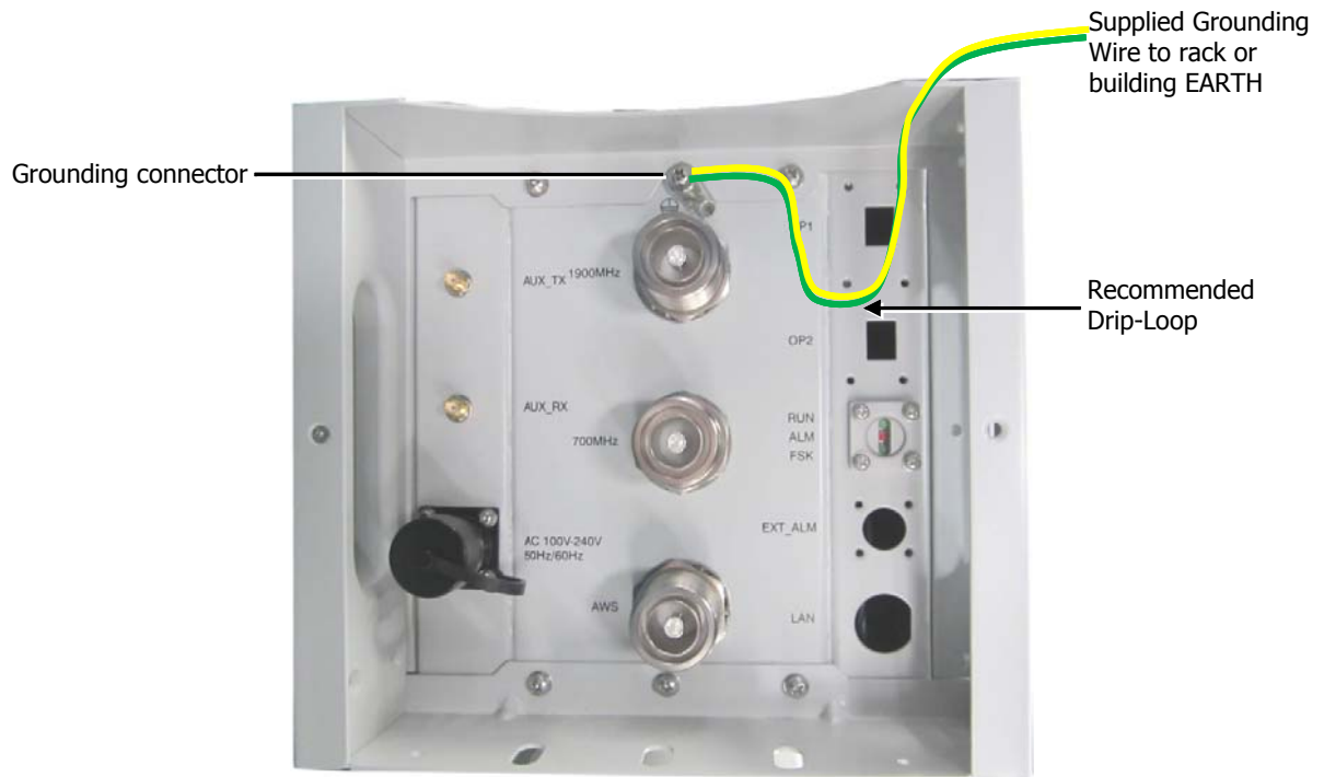
Figure 2-10. GX Grounding Connection
