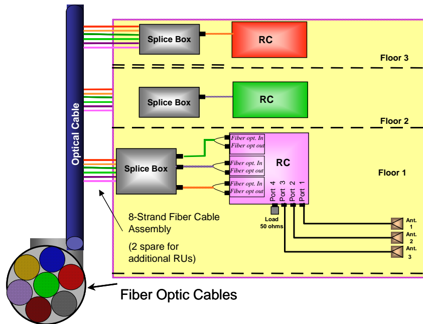
Figure 3-1. Illustration of Fiber Optic Routing
