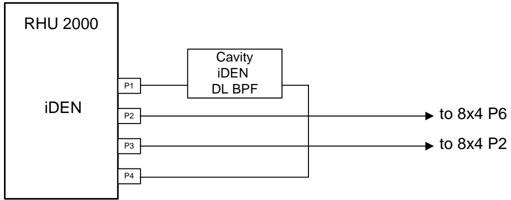
5-6. iDEN Configuration
