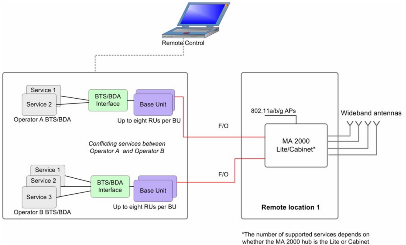
Figure 1-2. System Architecture
